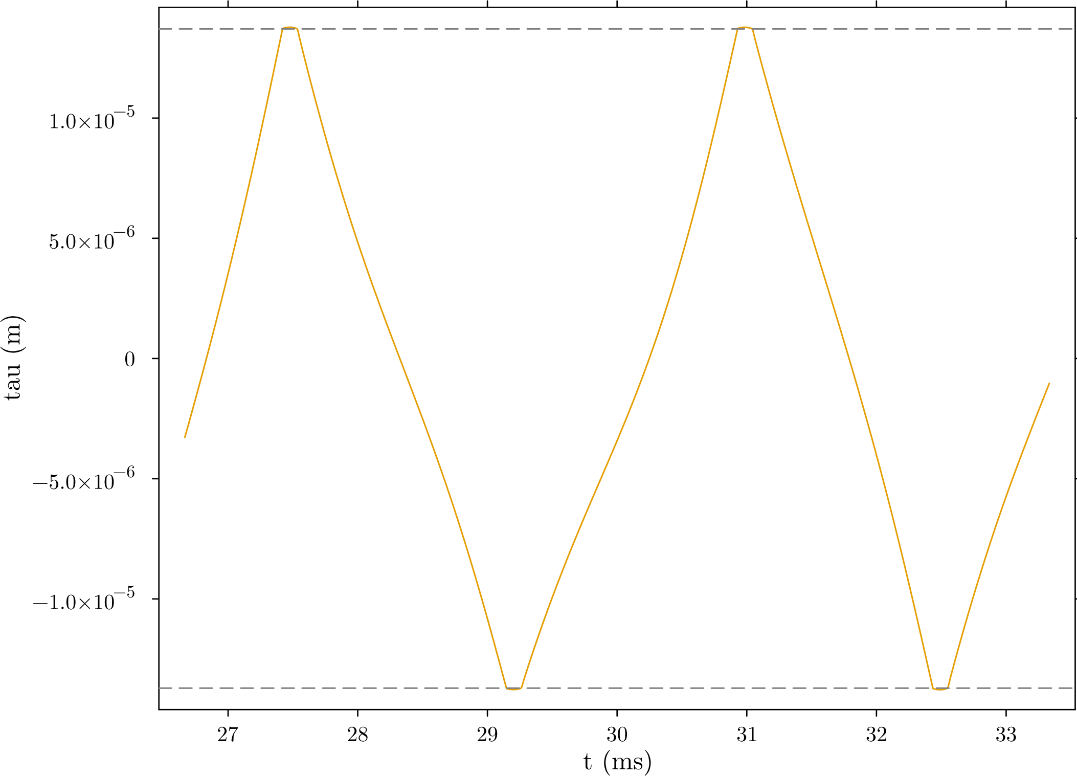
Compliant Tip Relative to its Stiff Face - last 2 cycles
