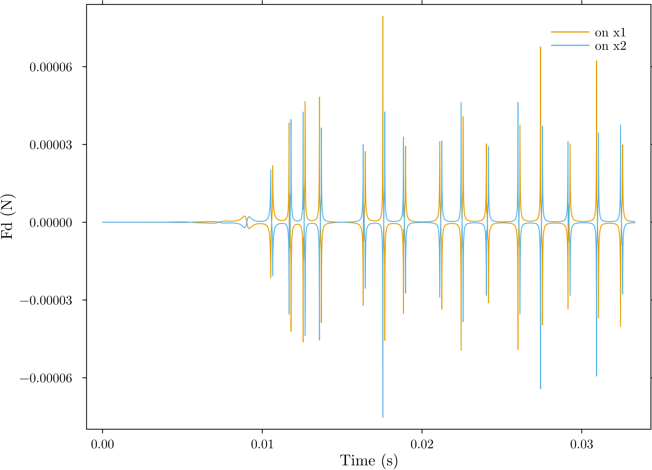
Squeeze-Film Force (projected Reynolds film)
