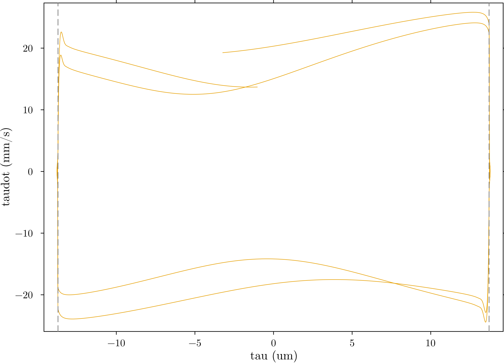
Tip Phase Plane - last 2 cycles
