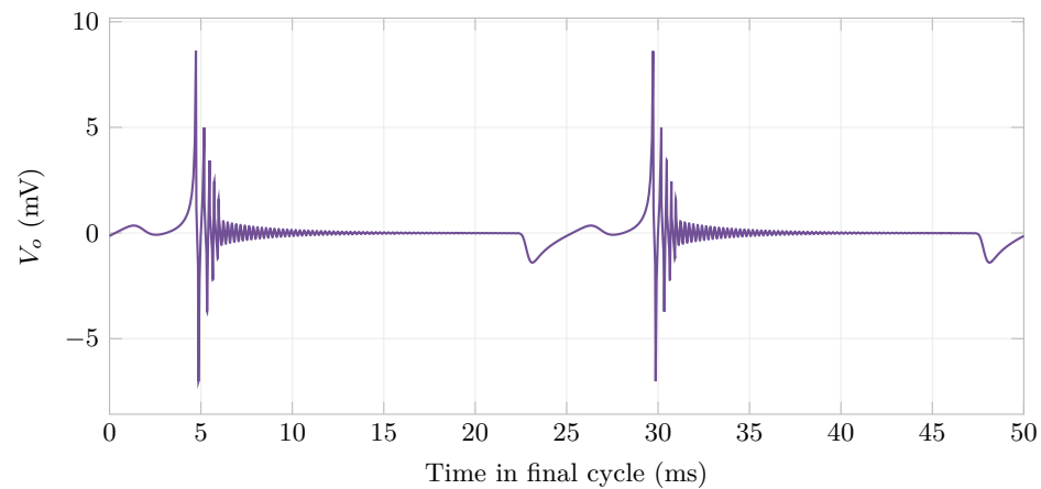
(b) Electrical output
