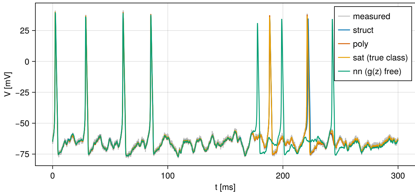
held-out, DC = 10, hidden = KCa
