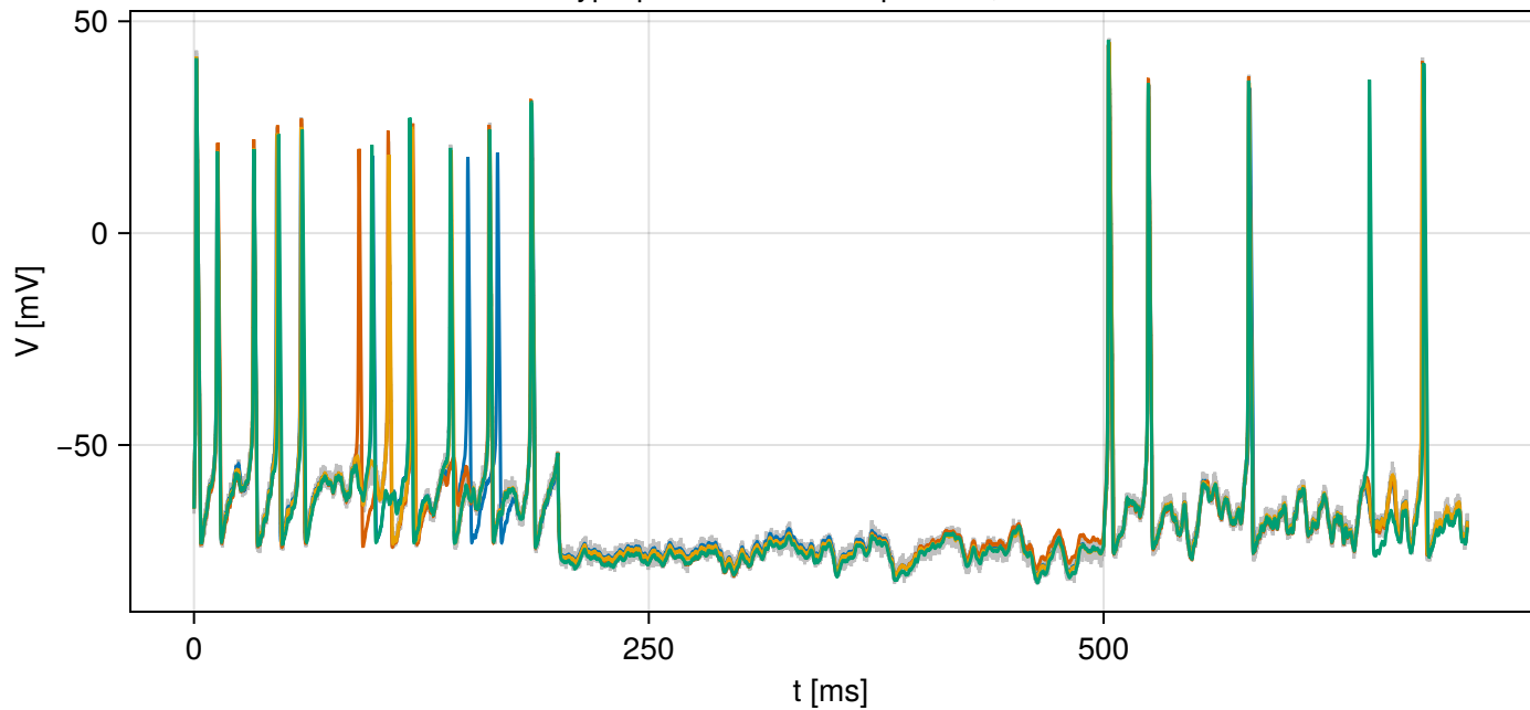
burst / hyperpolarise / release protocol, hidden = KCa
