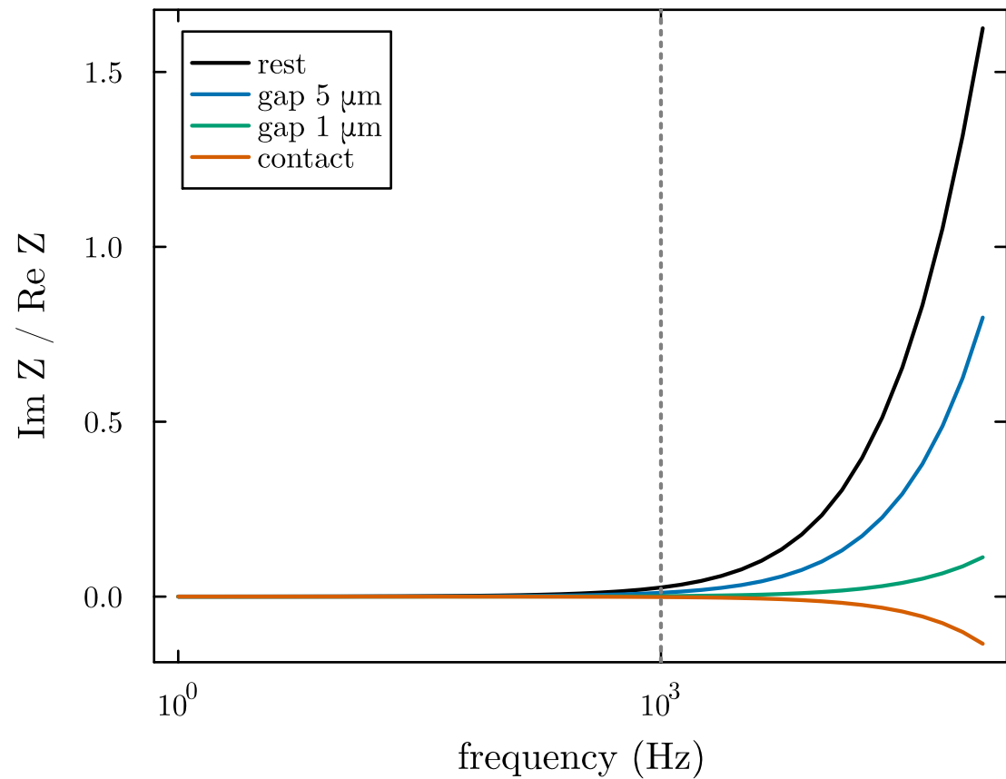
Reactance (+ mass-like, - spring-like)
