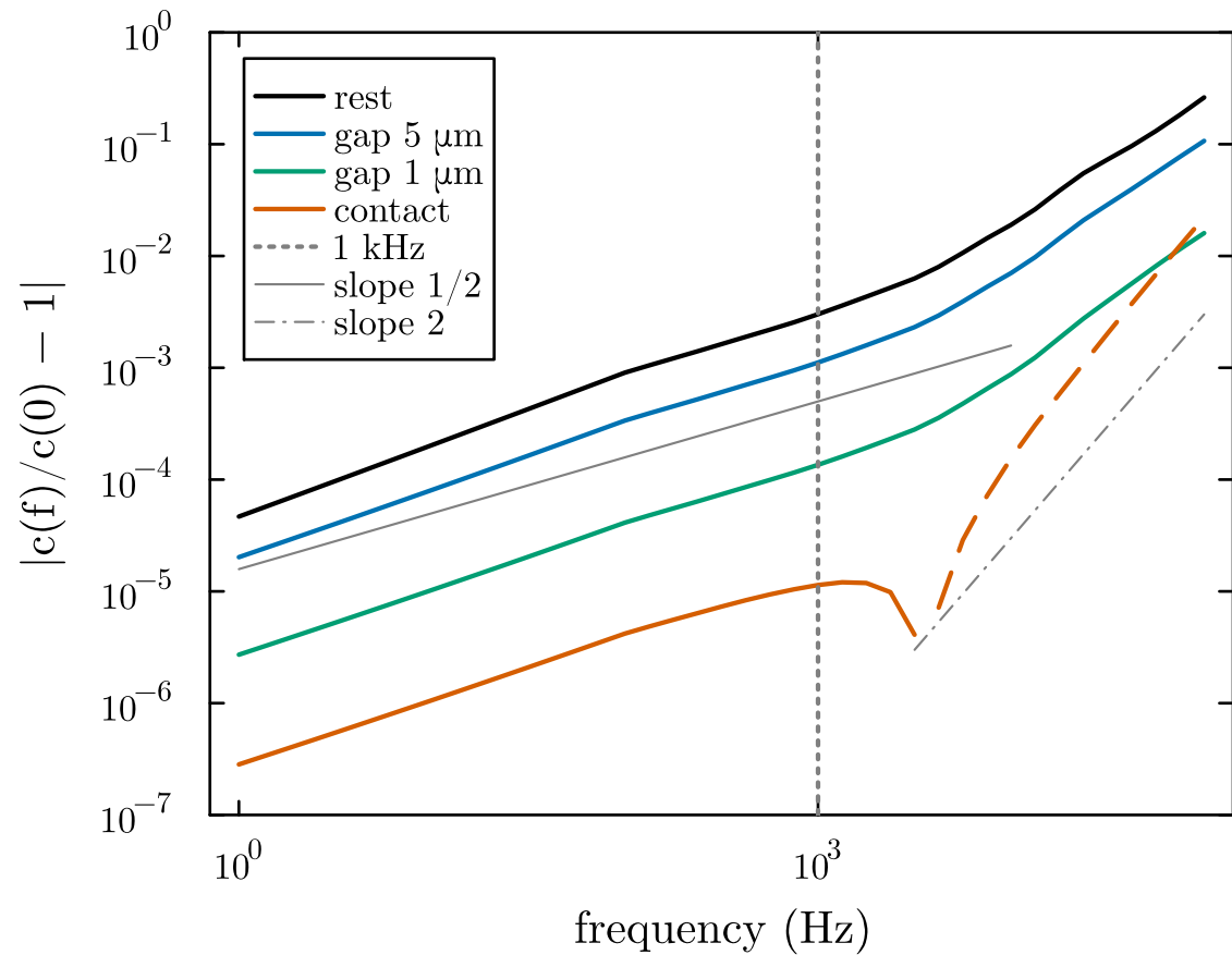
Damping change (dashed: decrease)
