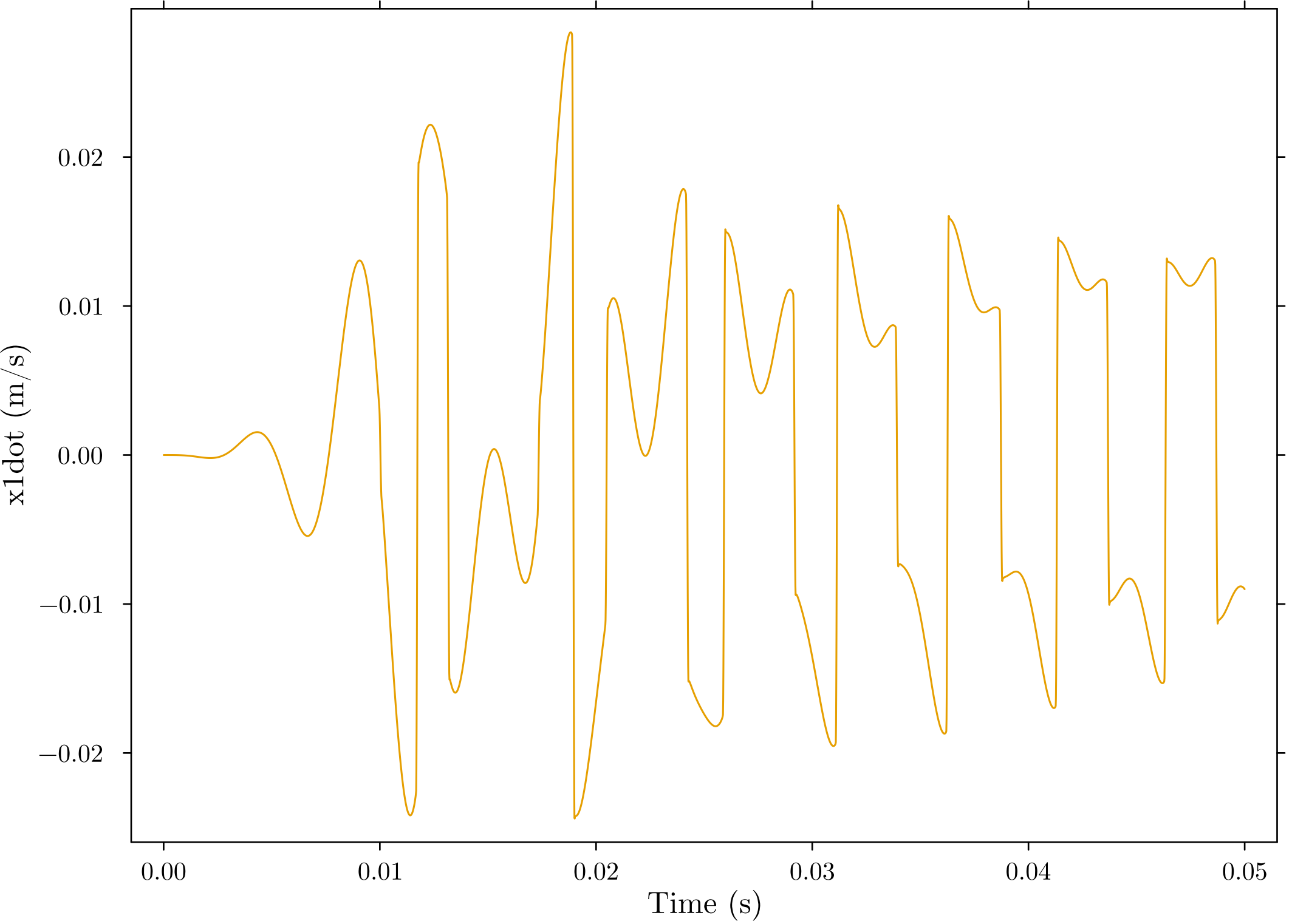
Shuttle Mass Velocity ( \dot{x}_1 )
