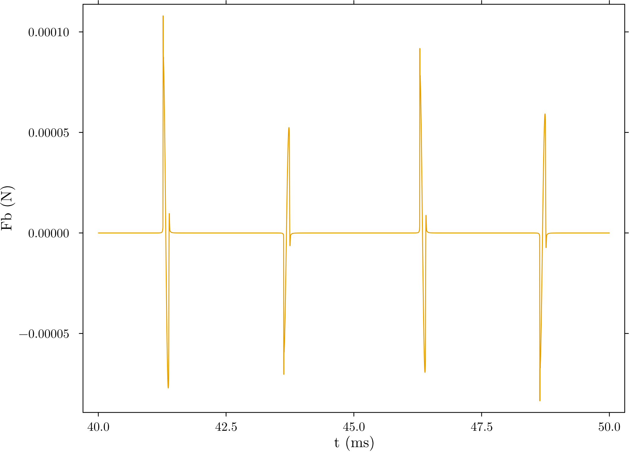
Beam Damping Force on the Tips - last 2 cycles
