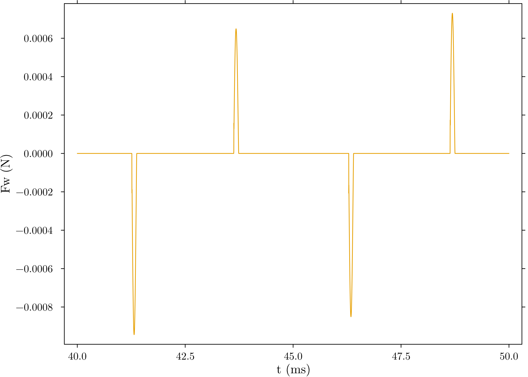
Tip Contact (Hunt-Crossley wall) Force - last 2 cycles
