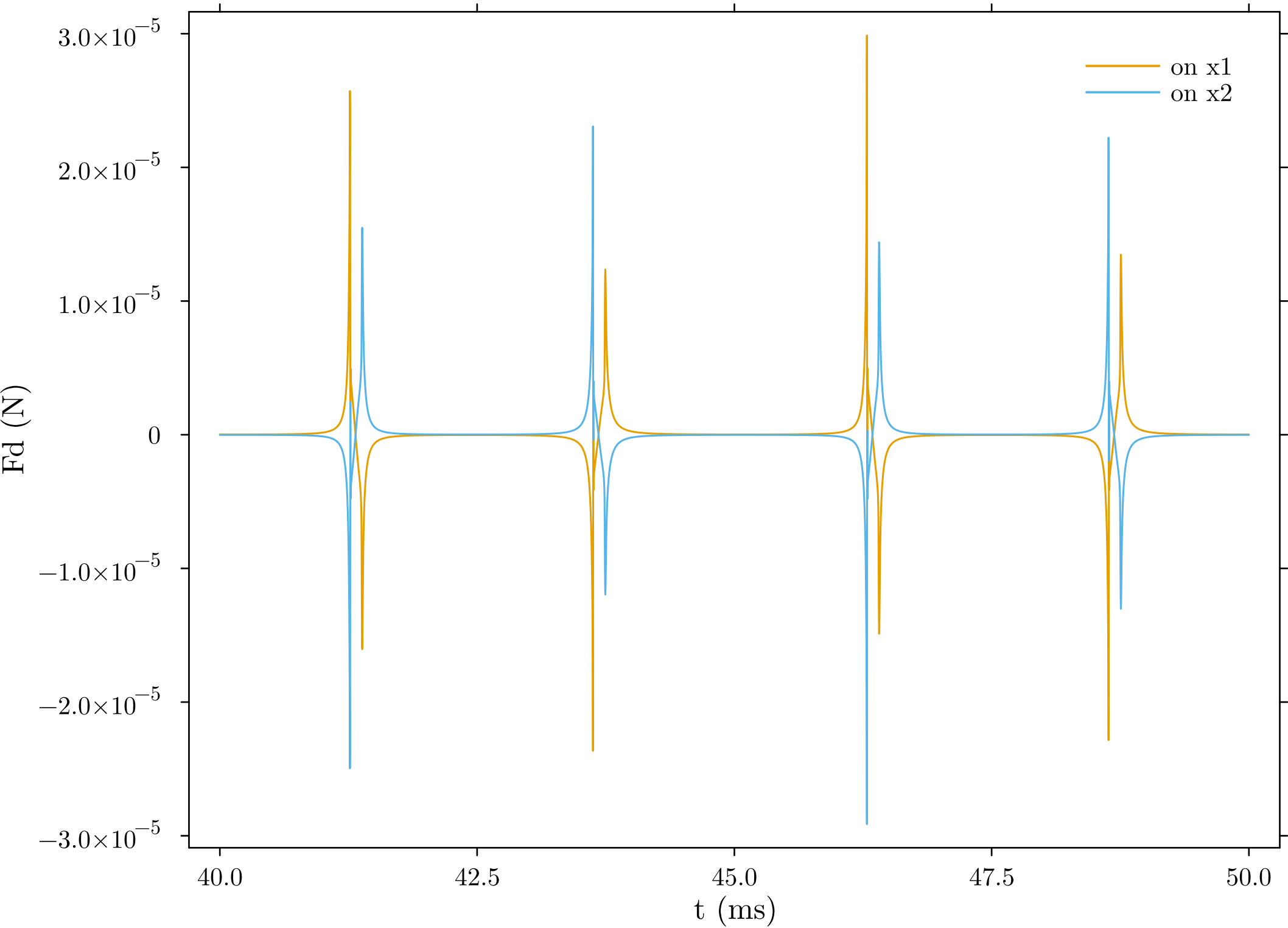
Squeeze-Film Force - last 2 cycles
