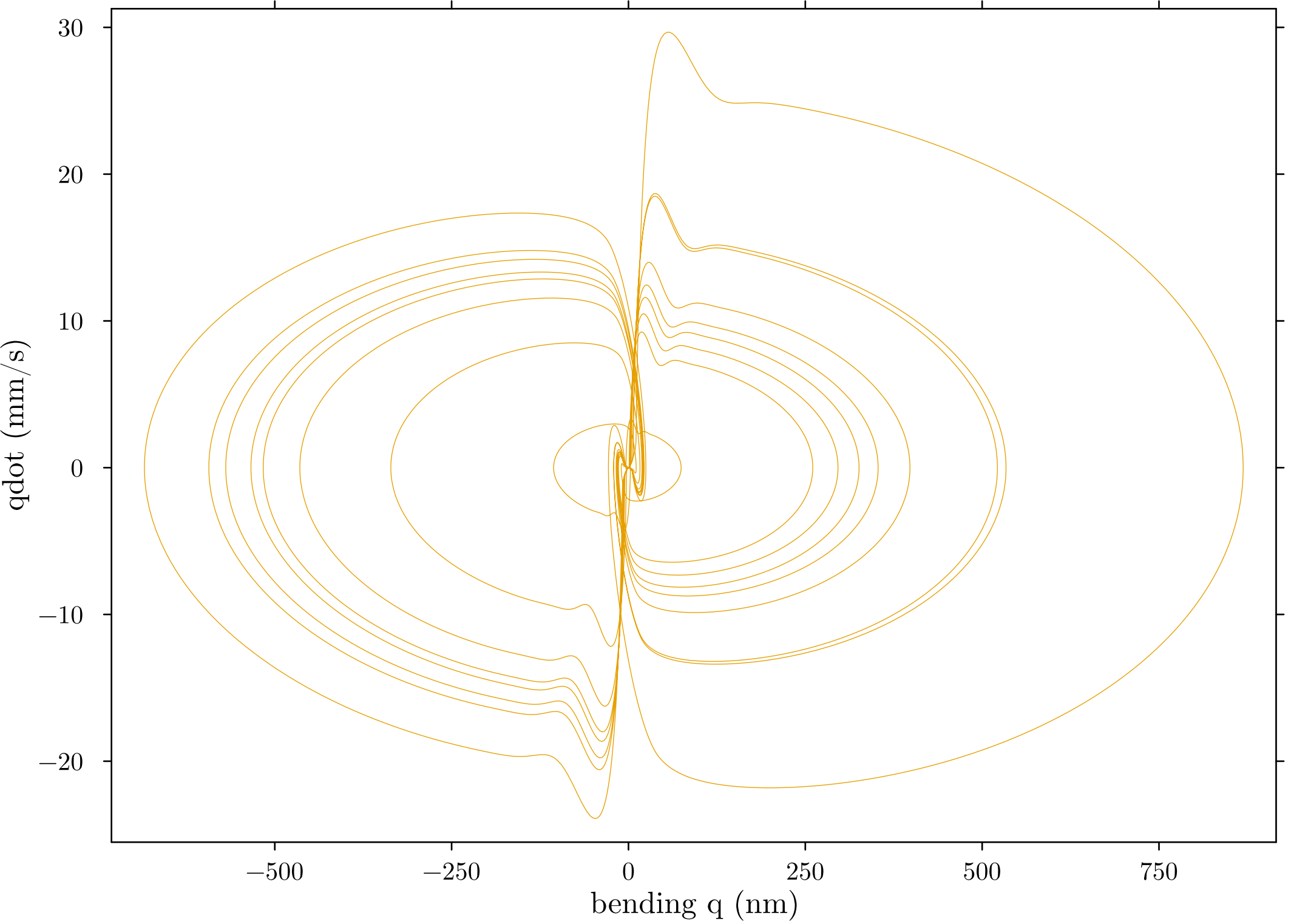
Electrode Bending Plane - full trajectory
