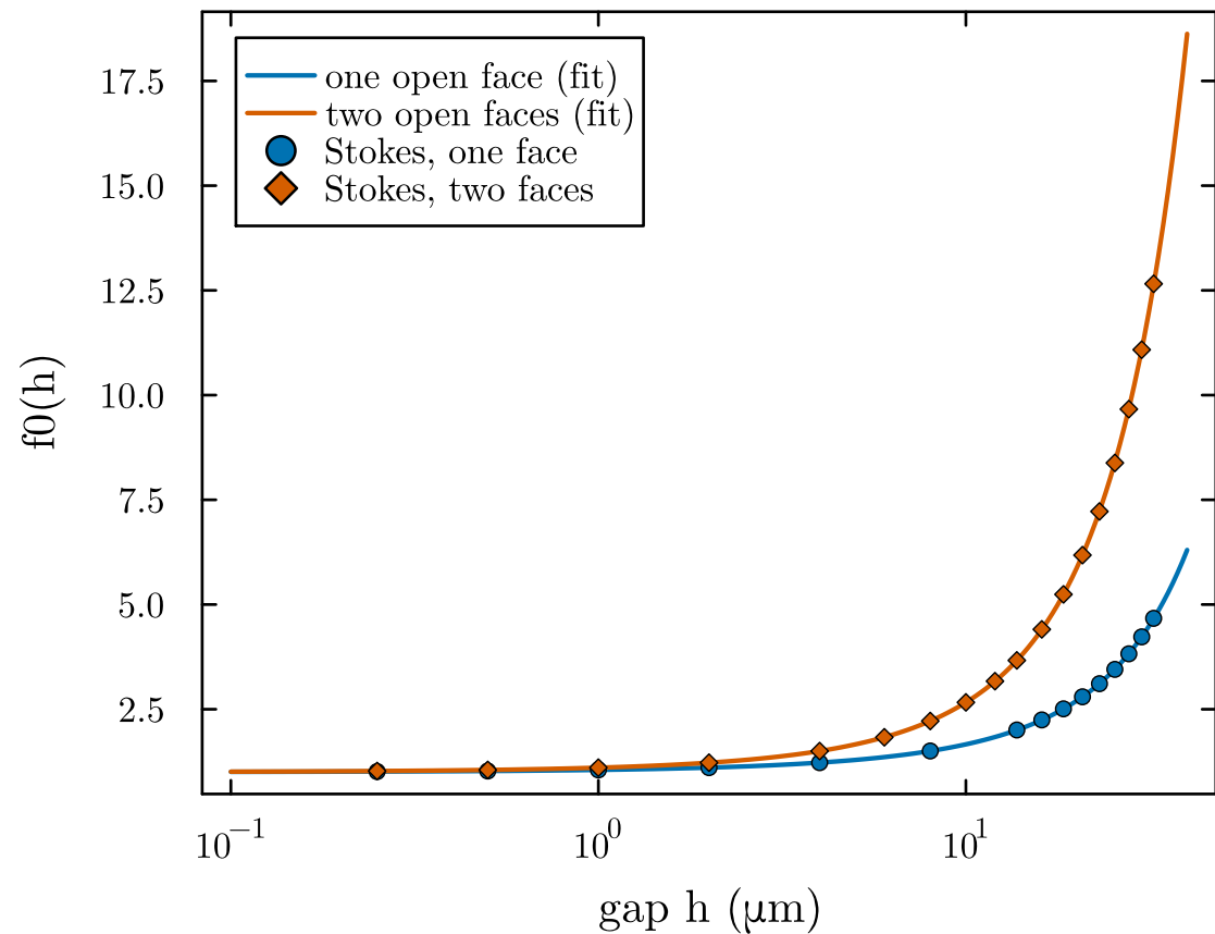
Lateral exit factor ( W = 25\text{ }\mu\text{m} )
