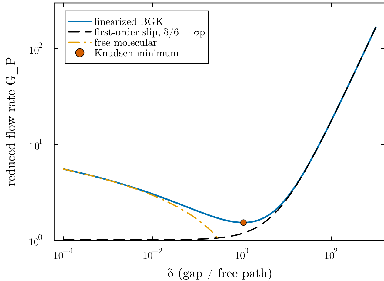
Plane Poiseuille flow of a rarefied gas
