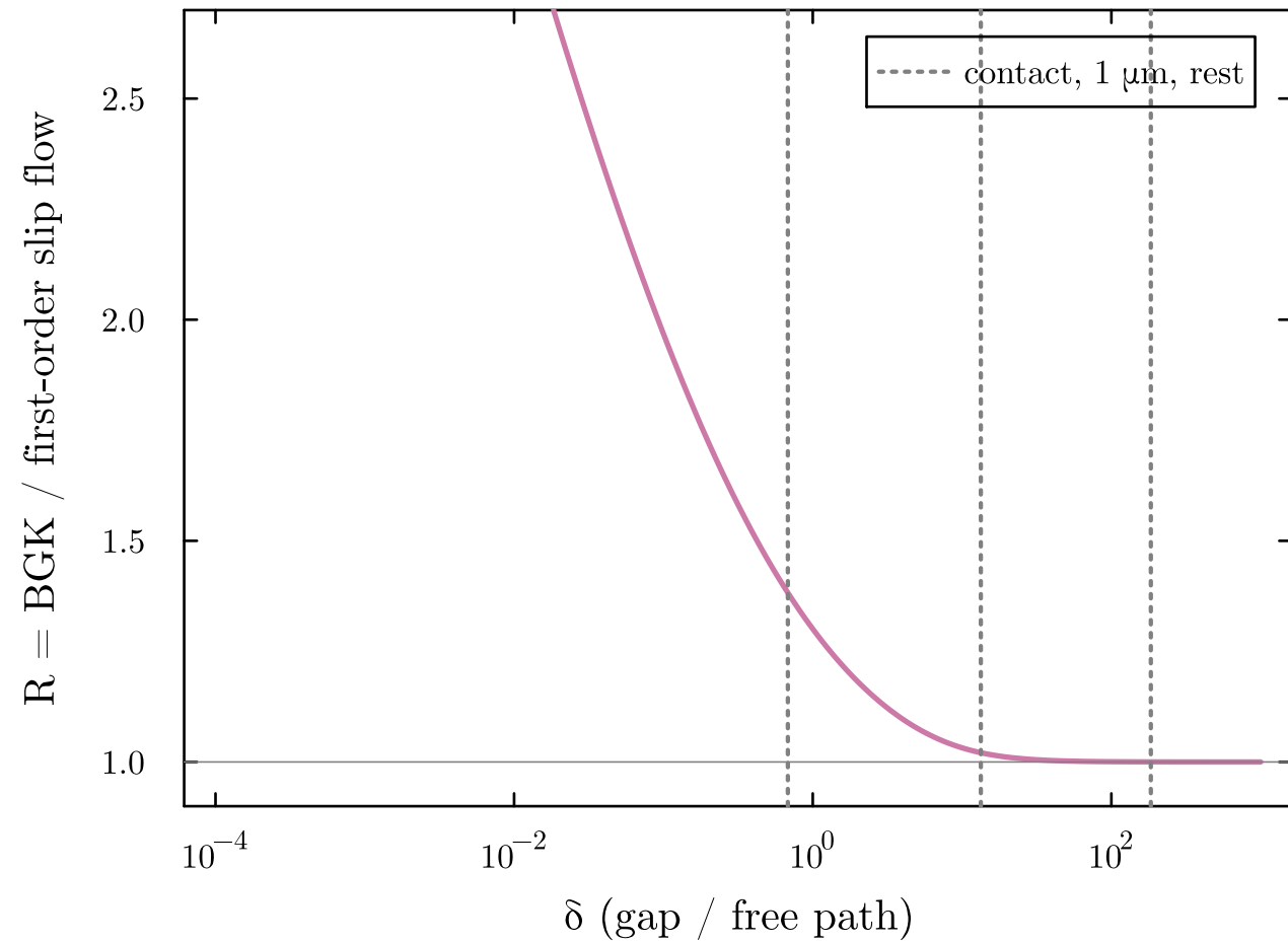
Kinetic flow factor
