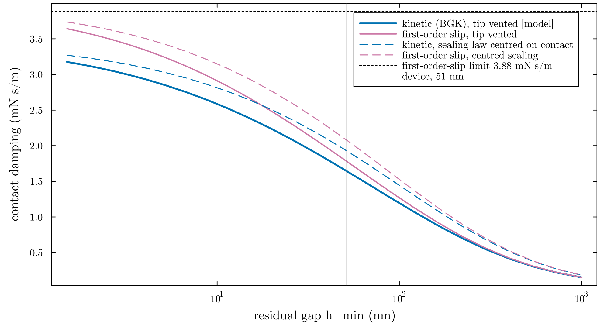
Contact damping: rarefaction and tip end condition (two open faces)
