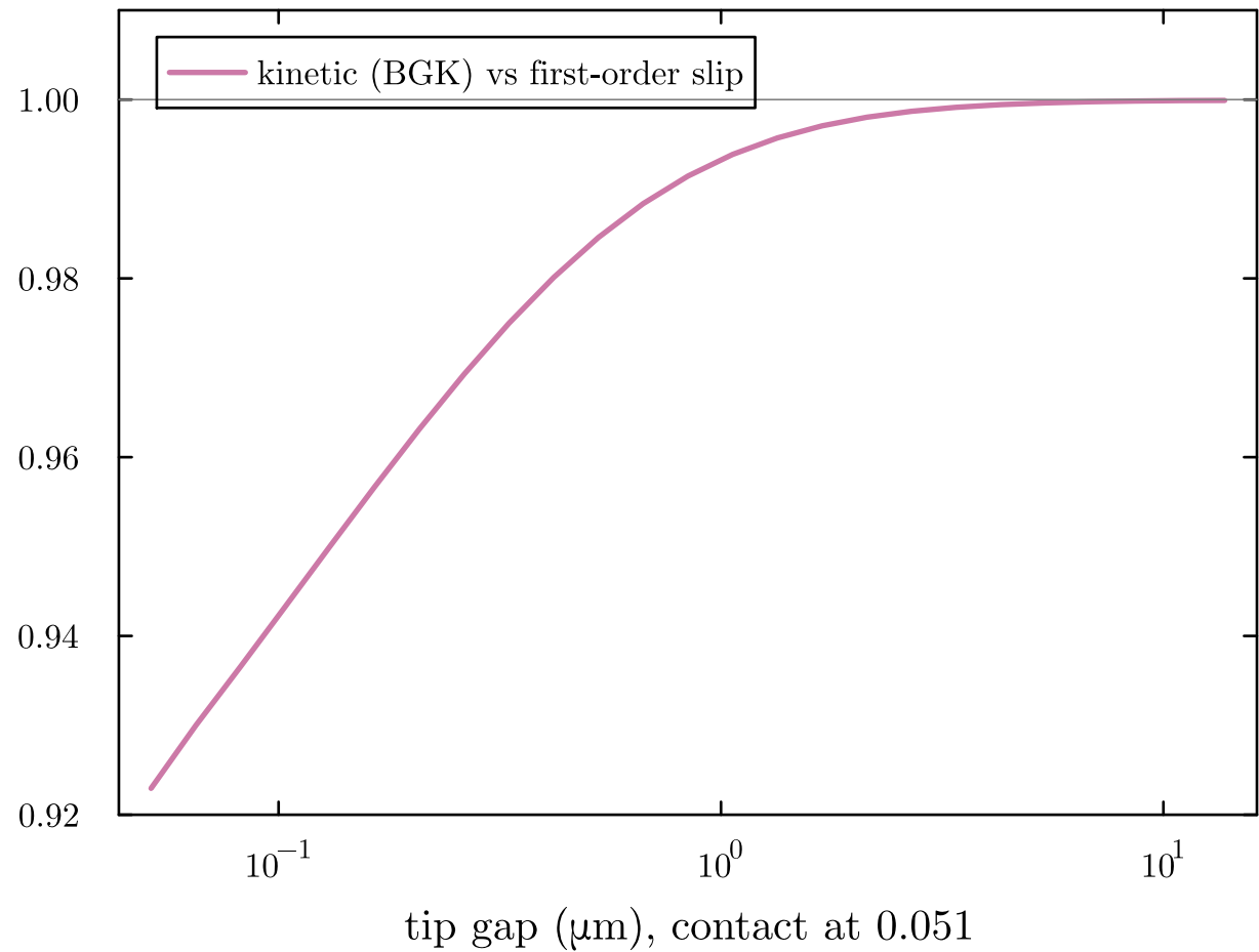
Rarefaction
