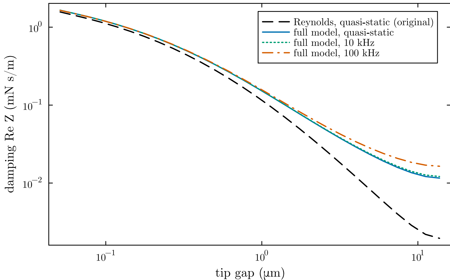
Damping across the stroke (two open faces)
