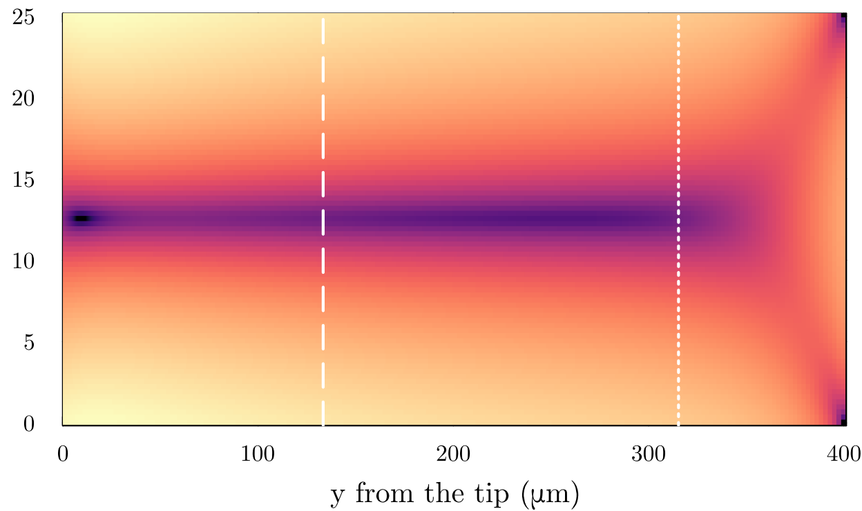
dissipation, rest: half within 133\ \mu\text{m} , 90% within 315\ \mu\text{m}
