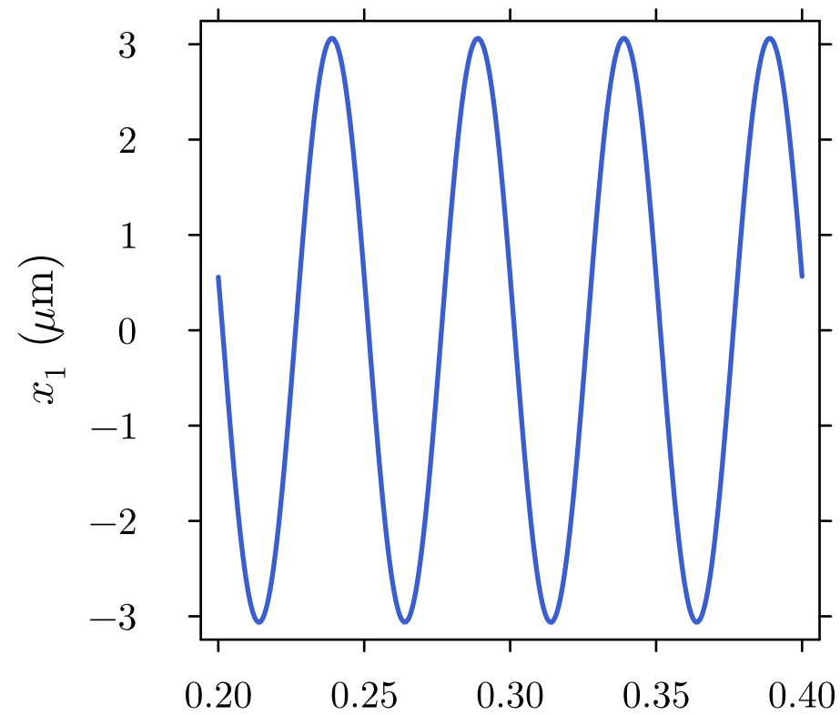
Shuttle Displacement
