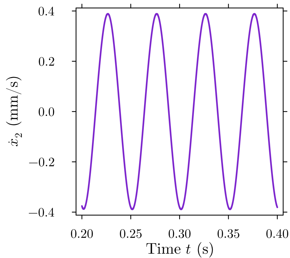
Electrode Velocity
