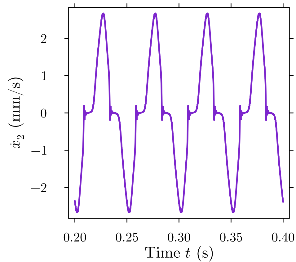
Electrode Velocity
