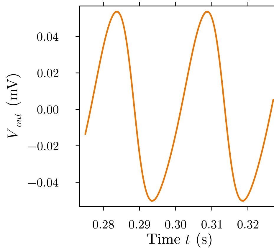
Output Voltage
