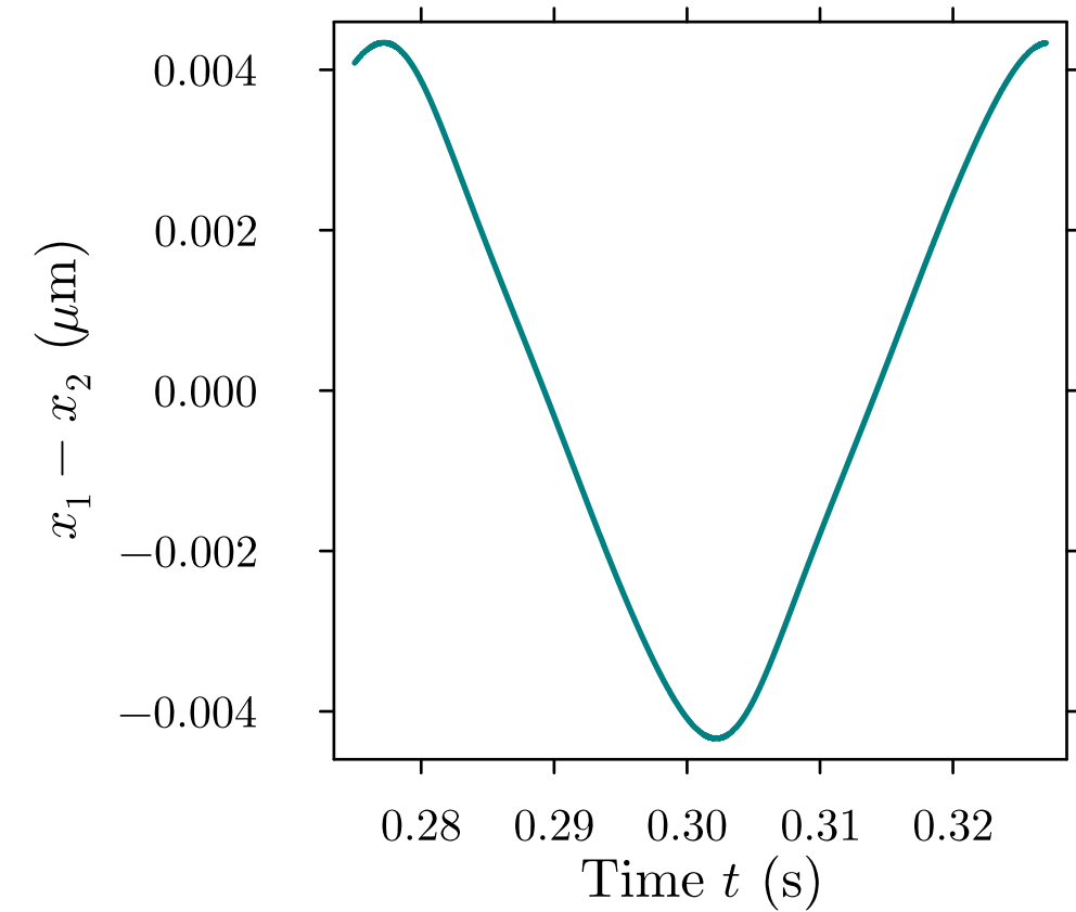
Relative Displacement
