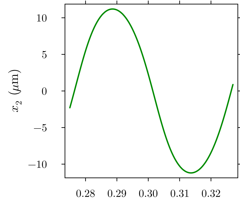
Electrode Displacement
