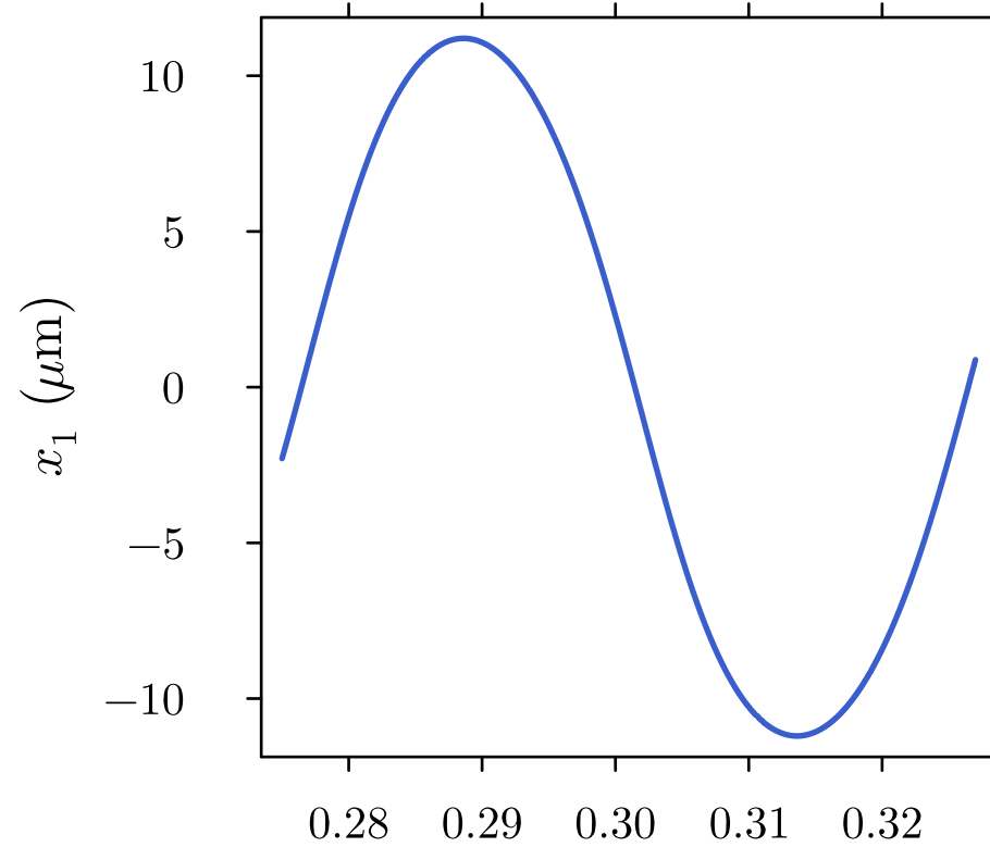
Shuttle Displacement
