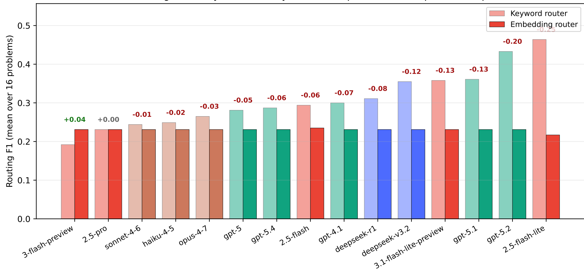
Embedding-similarity router vs keyword-overlap router (same planner outputs)
