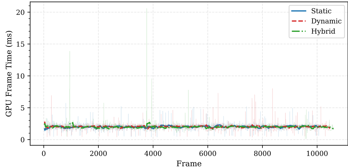
GPU Frame Time — 100 Boids
