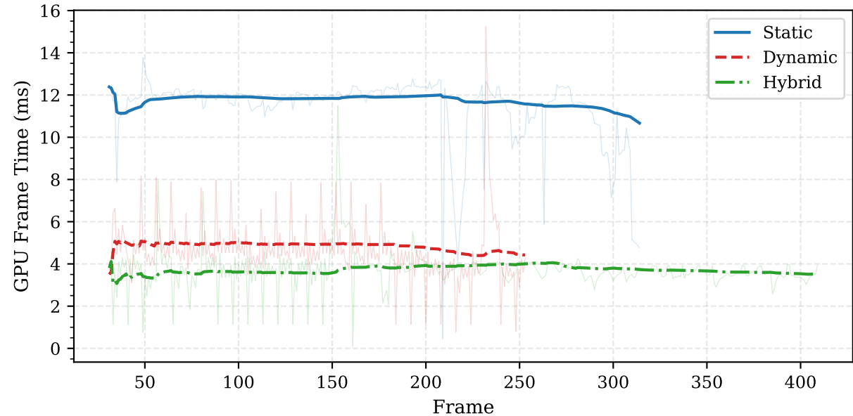
GPU Frame Time — 1000 Boids
