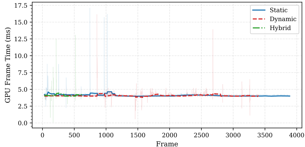
GPU Frame Time — 250 Boids
