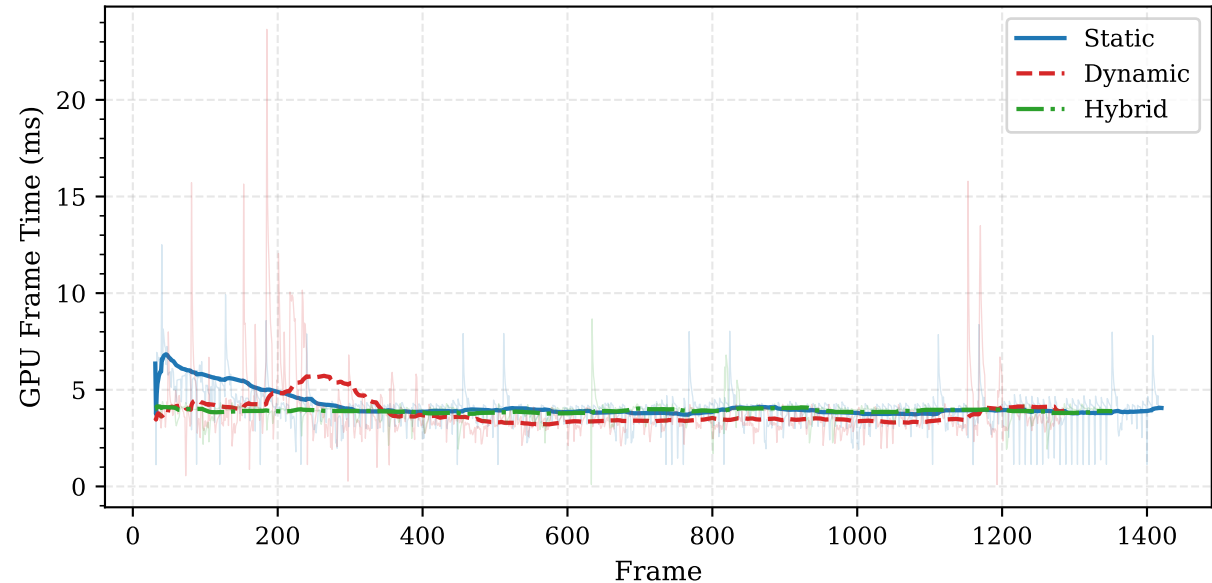
GPU Frame Time — 500 Boids
