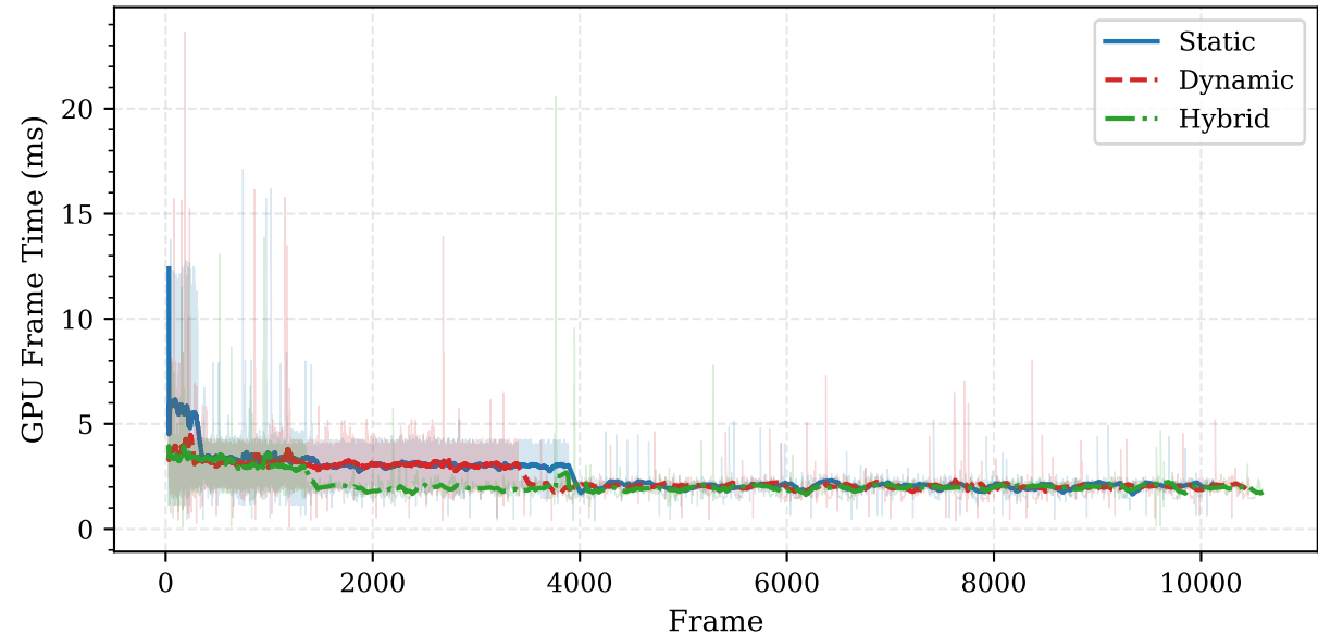
GPU Frame Time by Rendering Configuration
