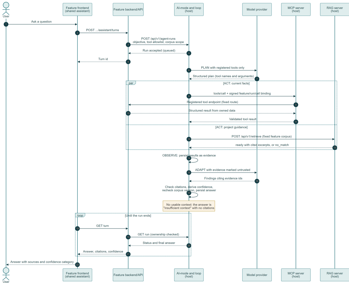
Figure 2 Frontend, backend, MCP and RAG interaction flow
