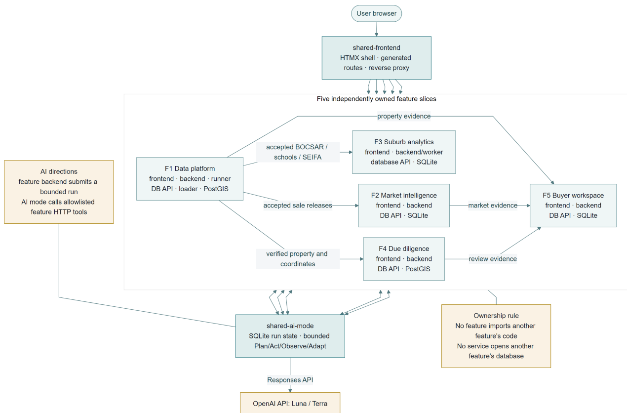
Figure 11 Integrated Release 0 software architecture
