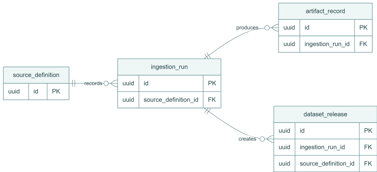
Figure 1 Feature 1 entity relationships and selected physical keys
