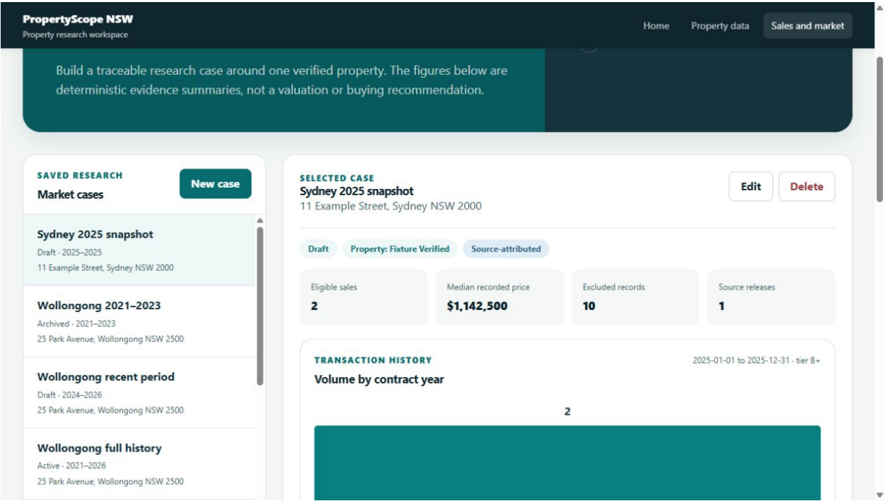
Figure 17 Feature 2 review of a deterministic market case
