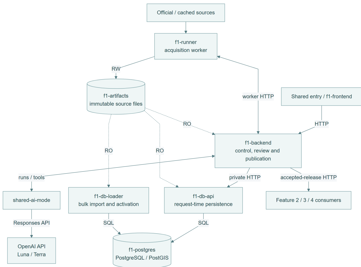
Figure 6 Feature 1 runtime trust boundaries acquisition loading AI callbacks and publication
