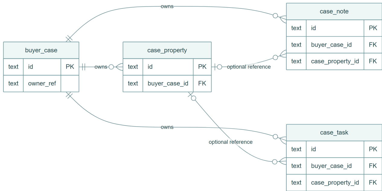
Figure 5 Feature 5 entity relationships and selected physical keys
