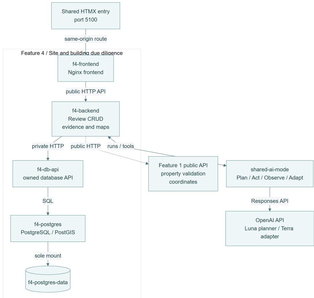
Figure 9 Feature 4 frontend backend persistence and AI boundaries
