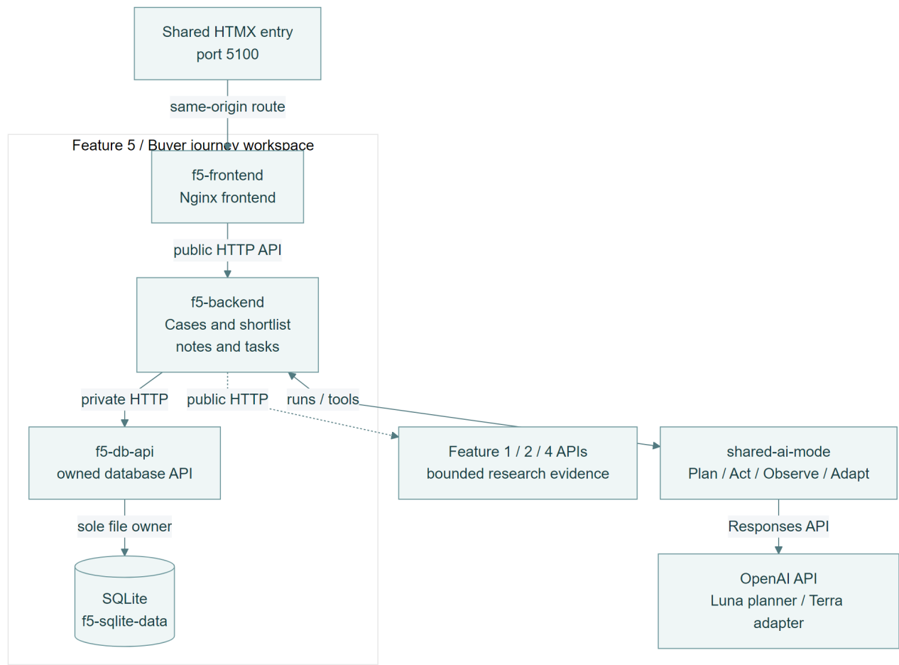
Figure 10 Feature 5 frontend backend persistence and AI boundaries
