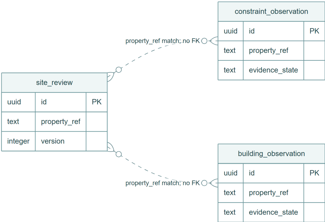
Figure 4 Feature 4 entity relationships and selected physical keys
