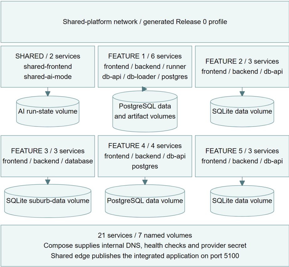
Figure 12 Docker Compose service groups
