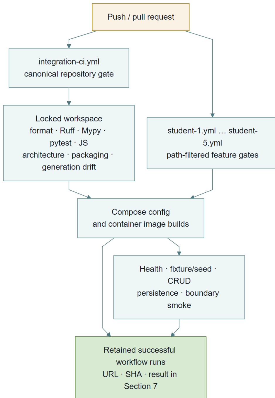
Figure 14 GitHub Actions and container validation pipeline
