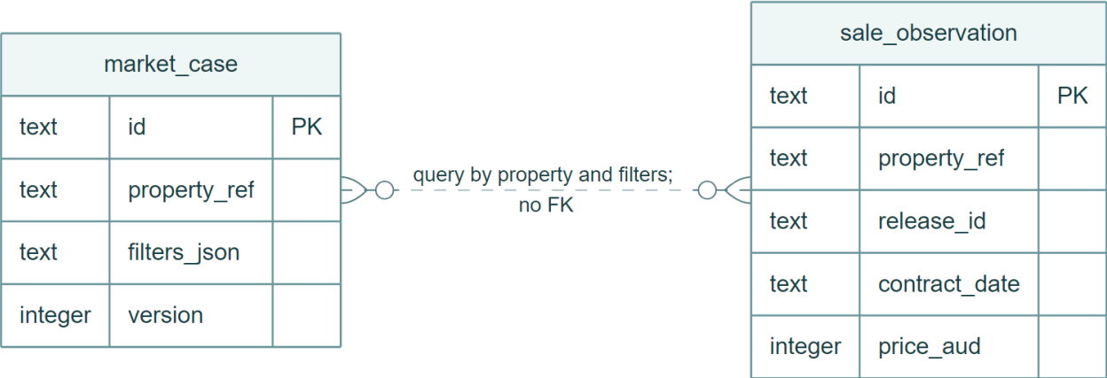
Figure 2 Feature 2 entity relationships and selected physical keys
