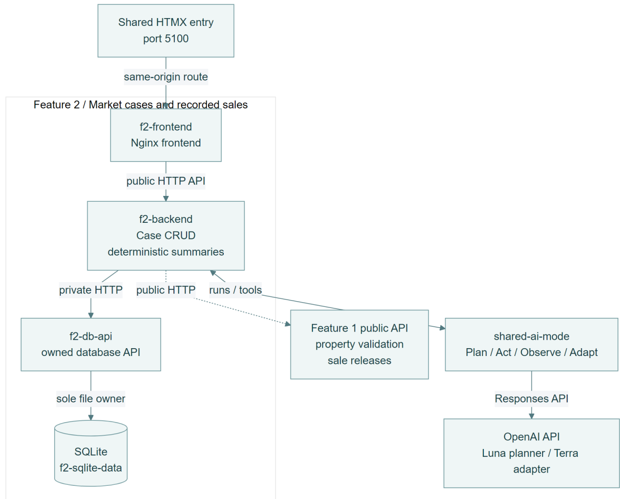
Figure 7 Feature 2 frontend backend persistence and AI boundaries
