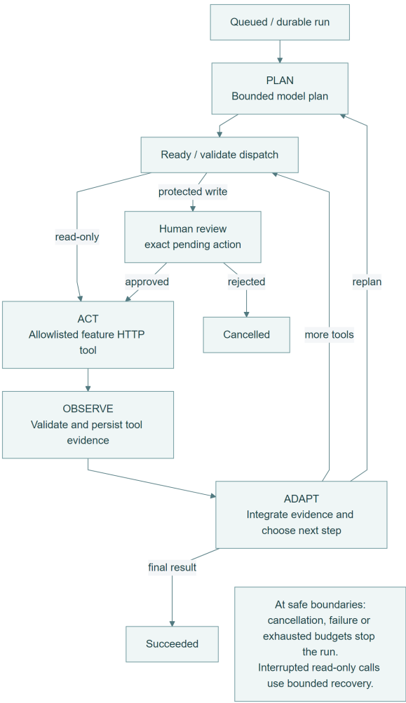
Figure 13 Bounded Plan Act Observe Adapt workflow
