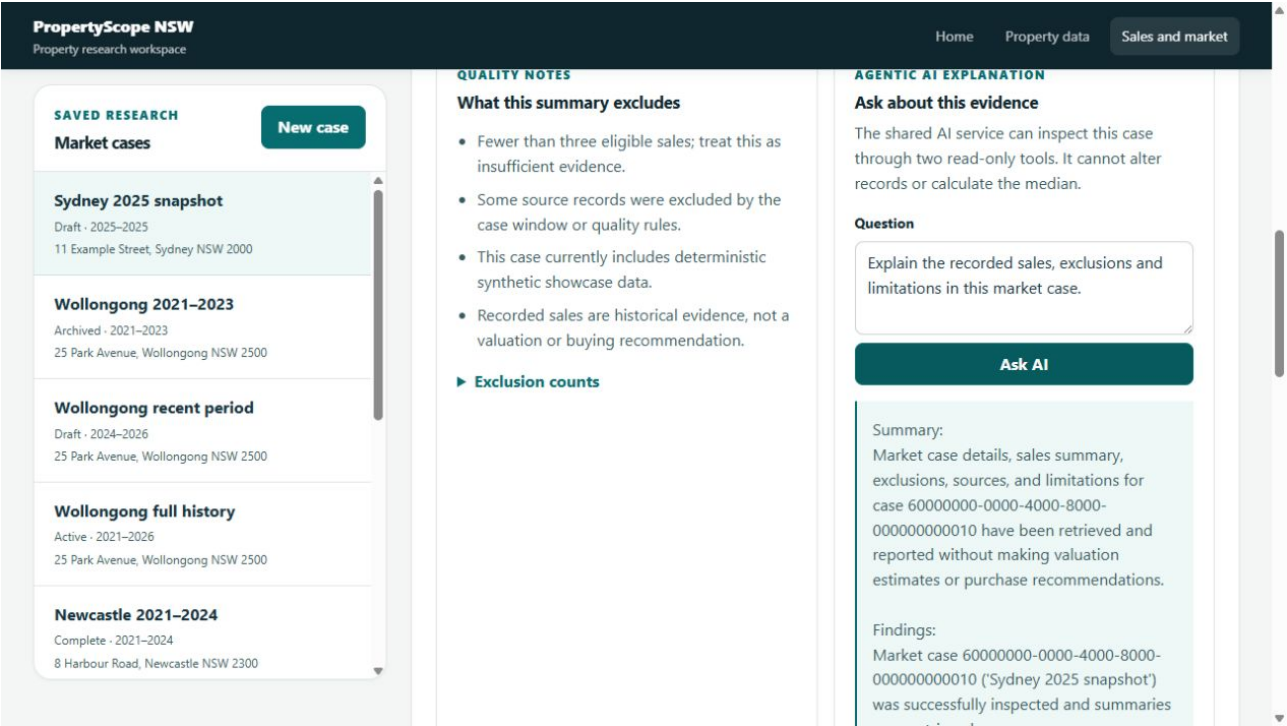
Figure 18 Feature 2 AI explanation of selected evidence
