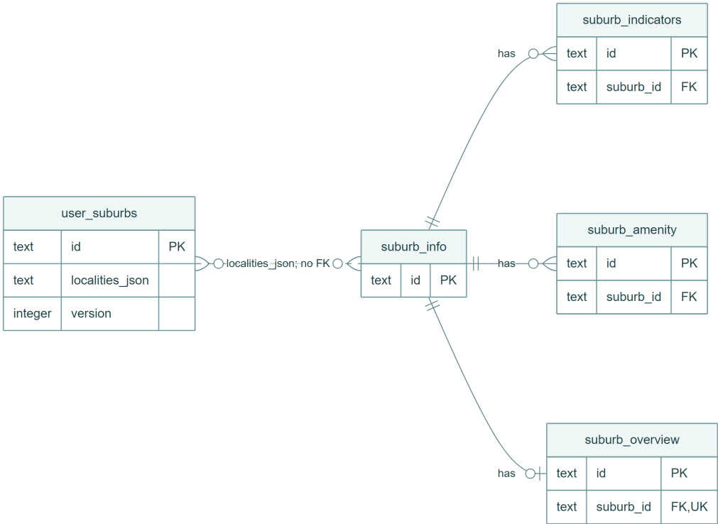
Figure 3 Feature 3 entity relationships and selected physical keys
