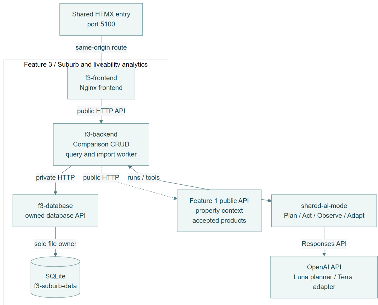
Figure 8 Feature 3 frontend backend persistence and AI boundaries
