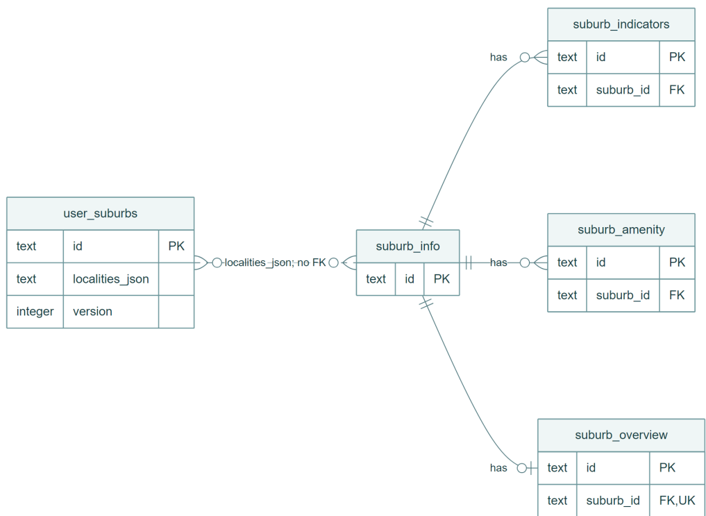
Figure 4 Feature 3 entity relationships and selected physical keys
