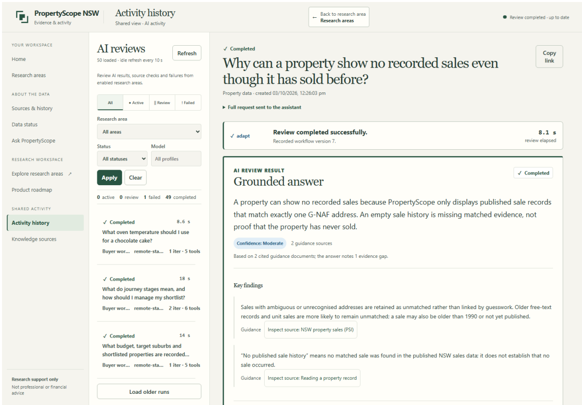
Figure 27 Cross-feature activity history
