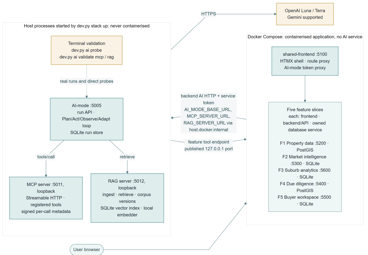
Figure 1 Overall Release 1 architecture and container boundary
