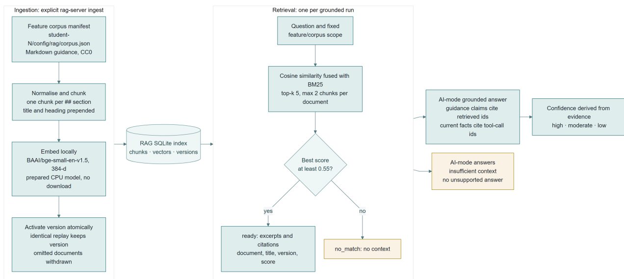
Figure 3 Versioned ingestion, retrieval and grounding
