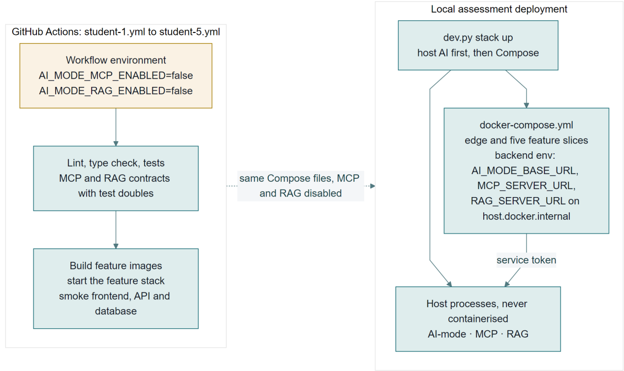
Figure 26 CI and local deployment
