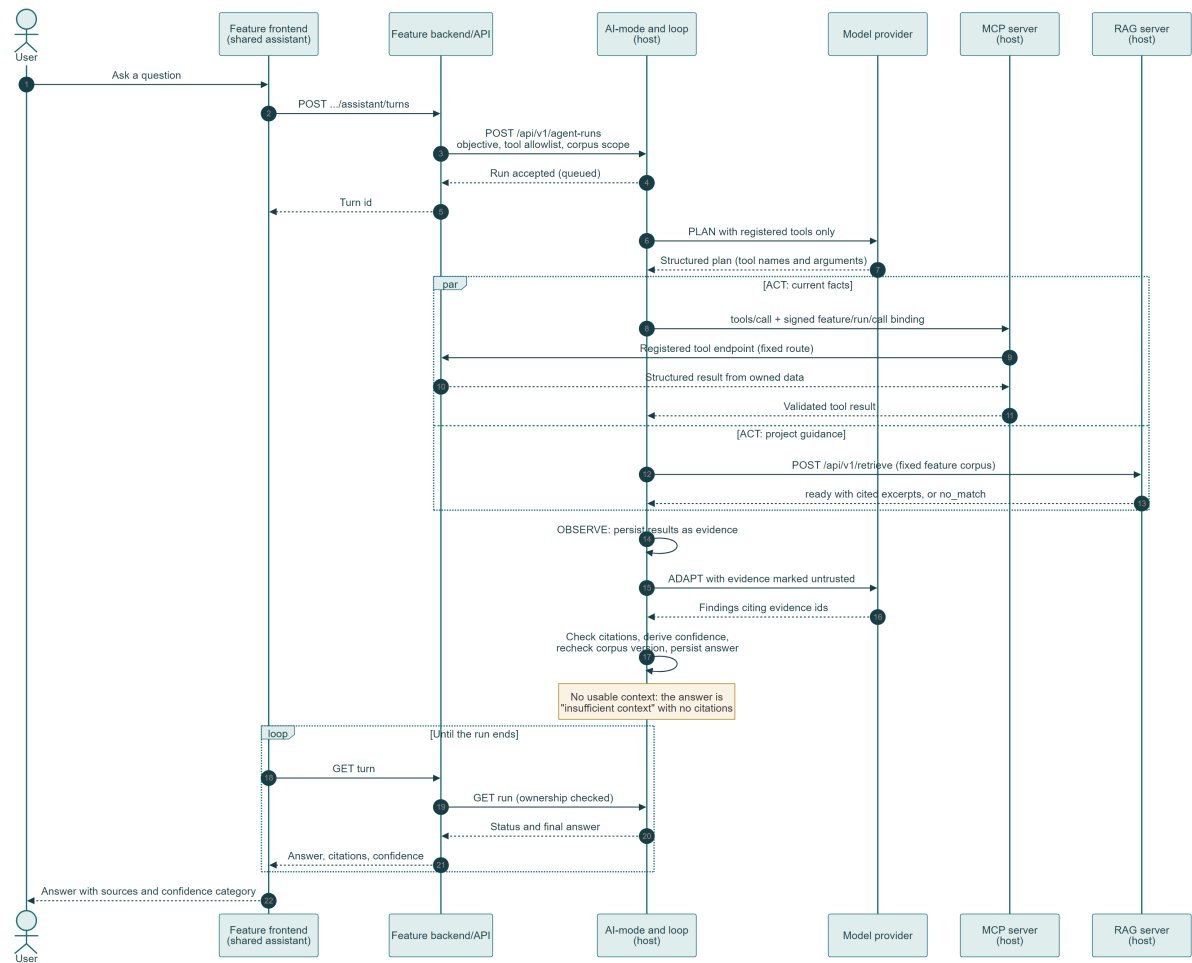
Figure 2 Frontend, backend, MCP and RAG interaction flow
