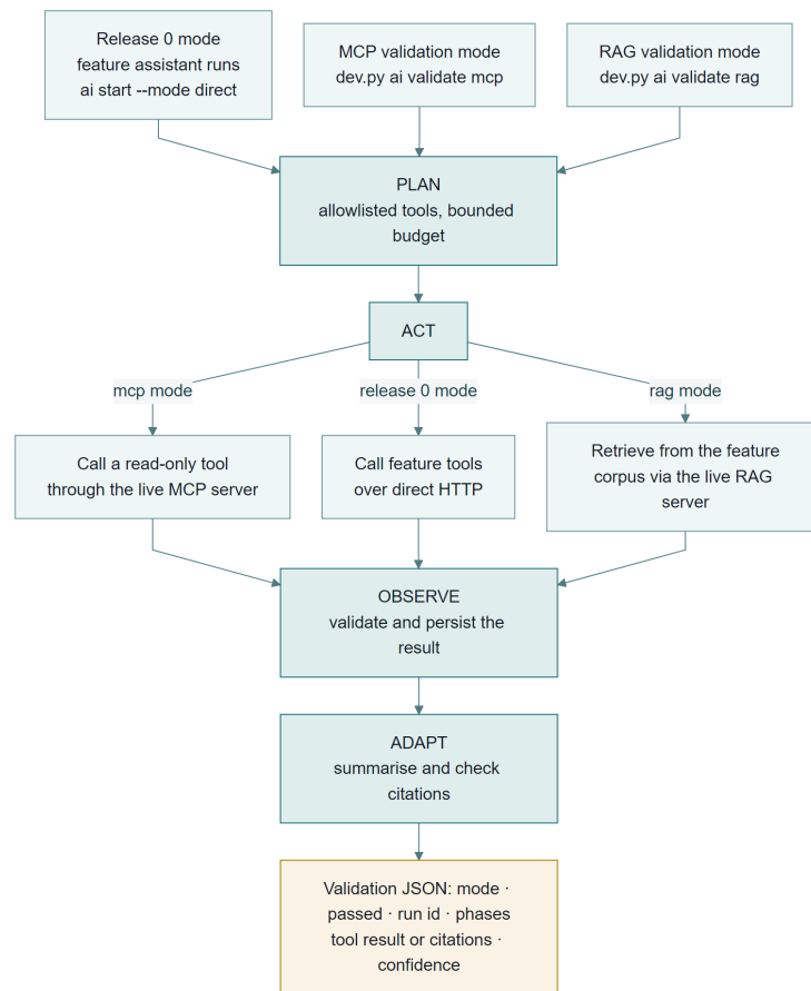
Figure 5 Loop entry points and validation modes
