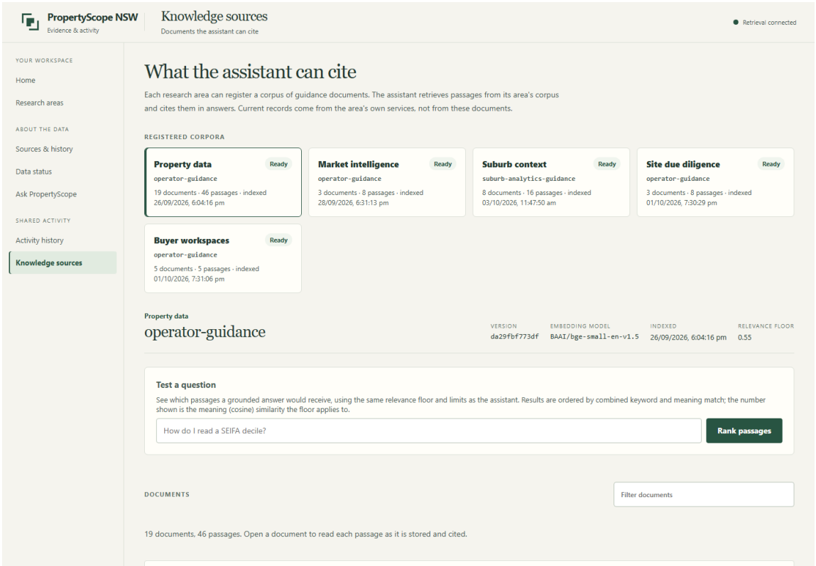
Figure 4 Registered knowledge sources in the running application
