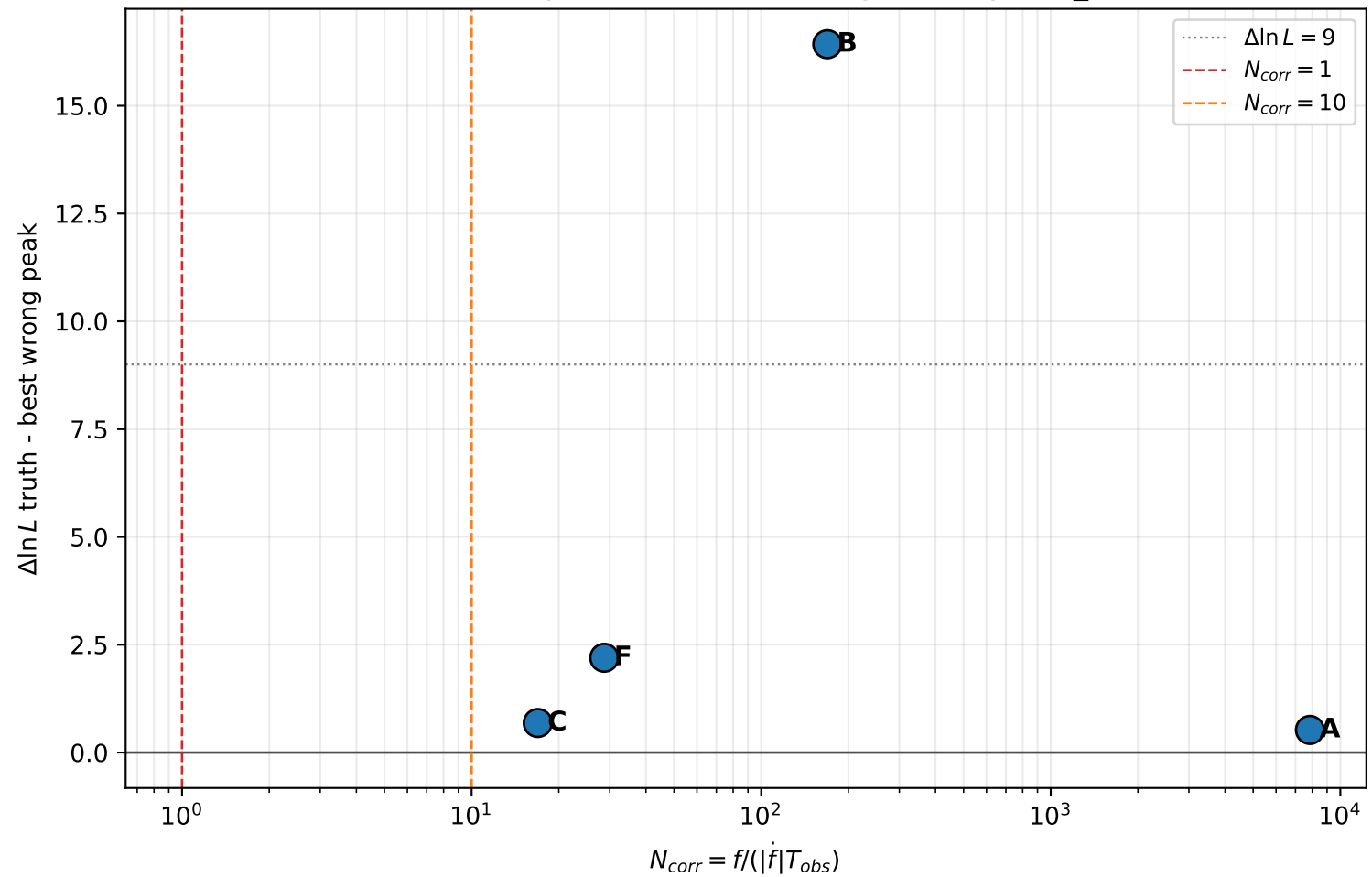
Measured single-CW mode breaking vs analytic N_corr
