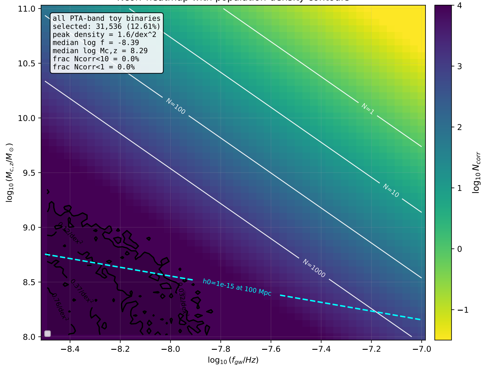
Part F1: All toy SMBHBs in the PTA band Ncorr heatmap with population-density contours
