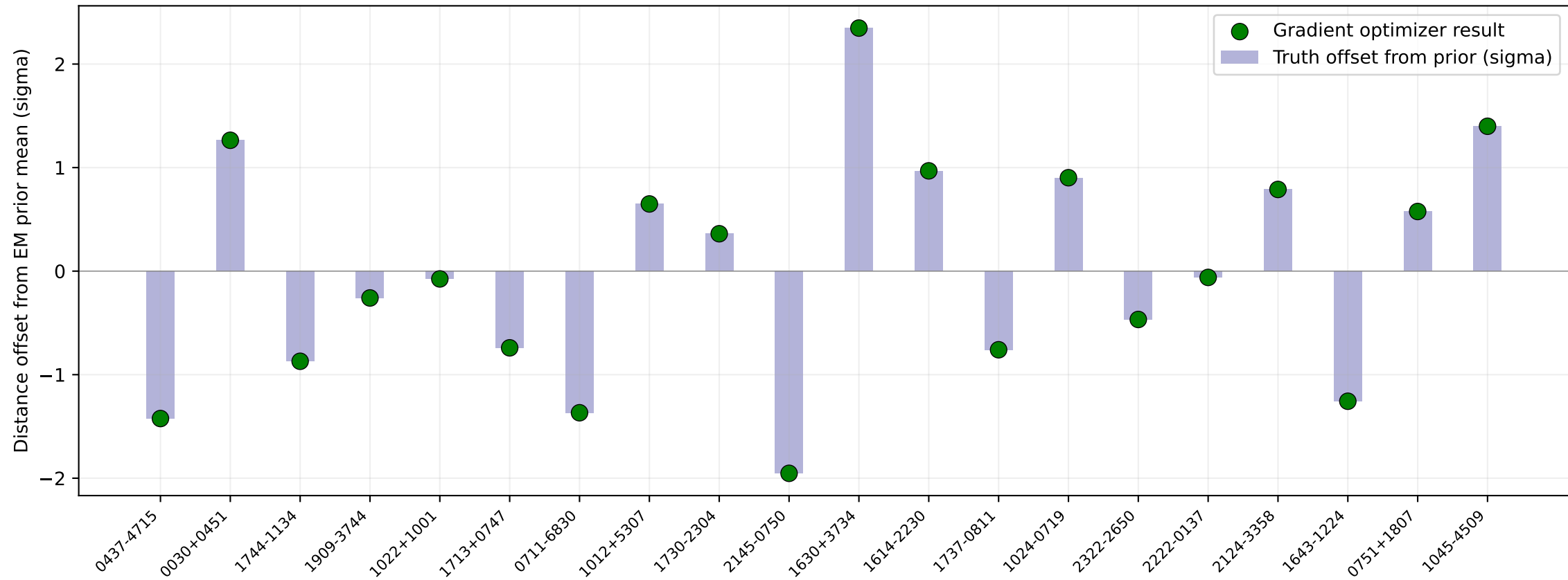
Pulsar Distance Recovery: 20/20 recovered best lnL = 105246.4 vs truth lnL = 105246.4 (Delta = 0.0)
