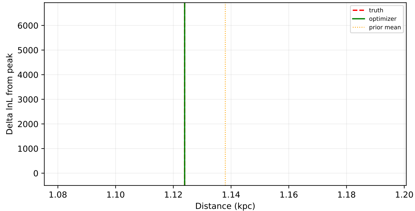
J1713+0747 (example)
