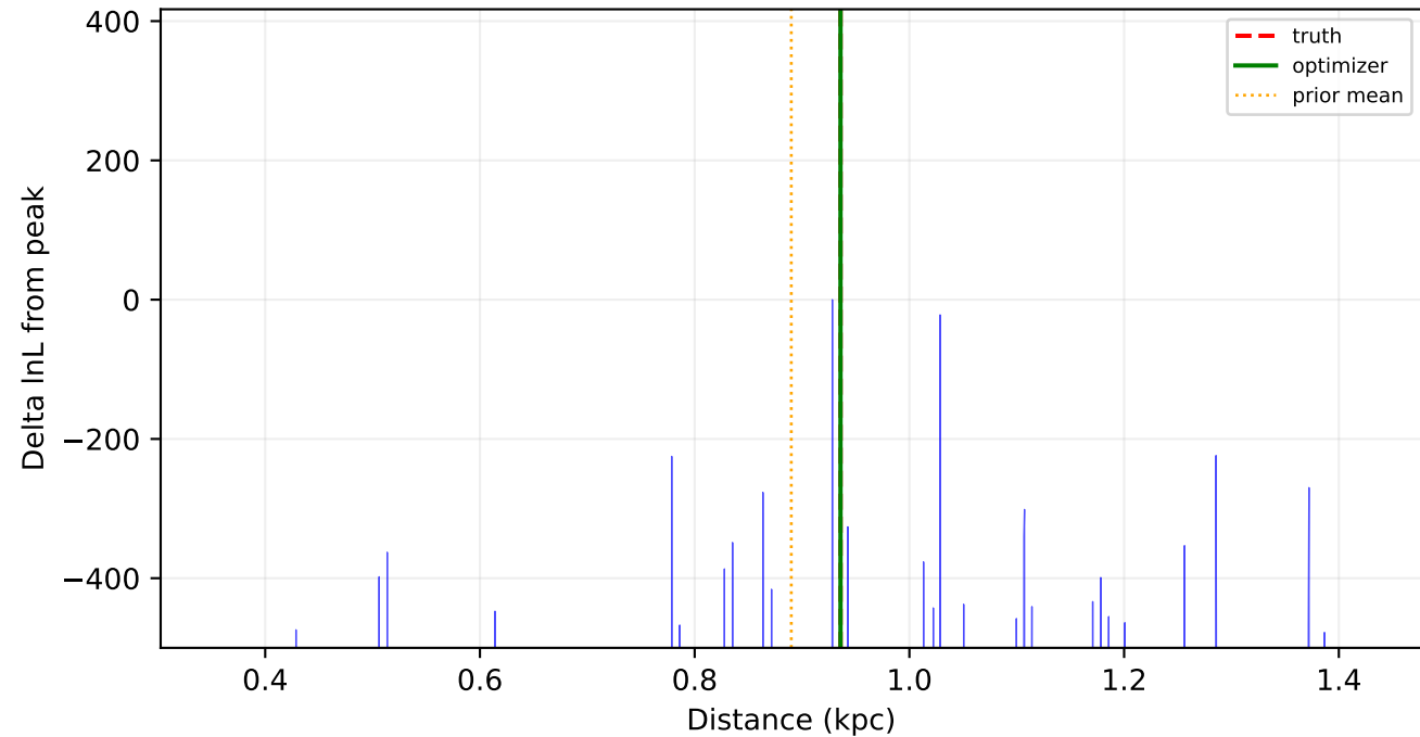
J0900-3144 (hardest)
