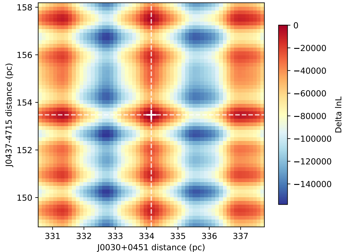
Other pulsars at truth
