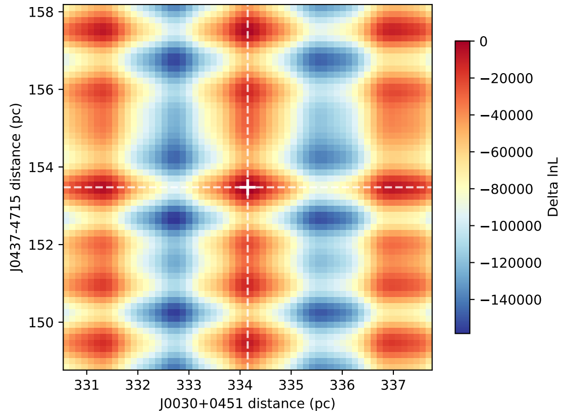
Other pulsars at optimizer result
