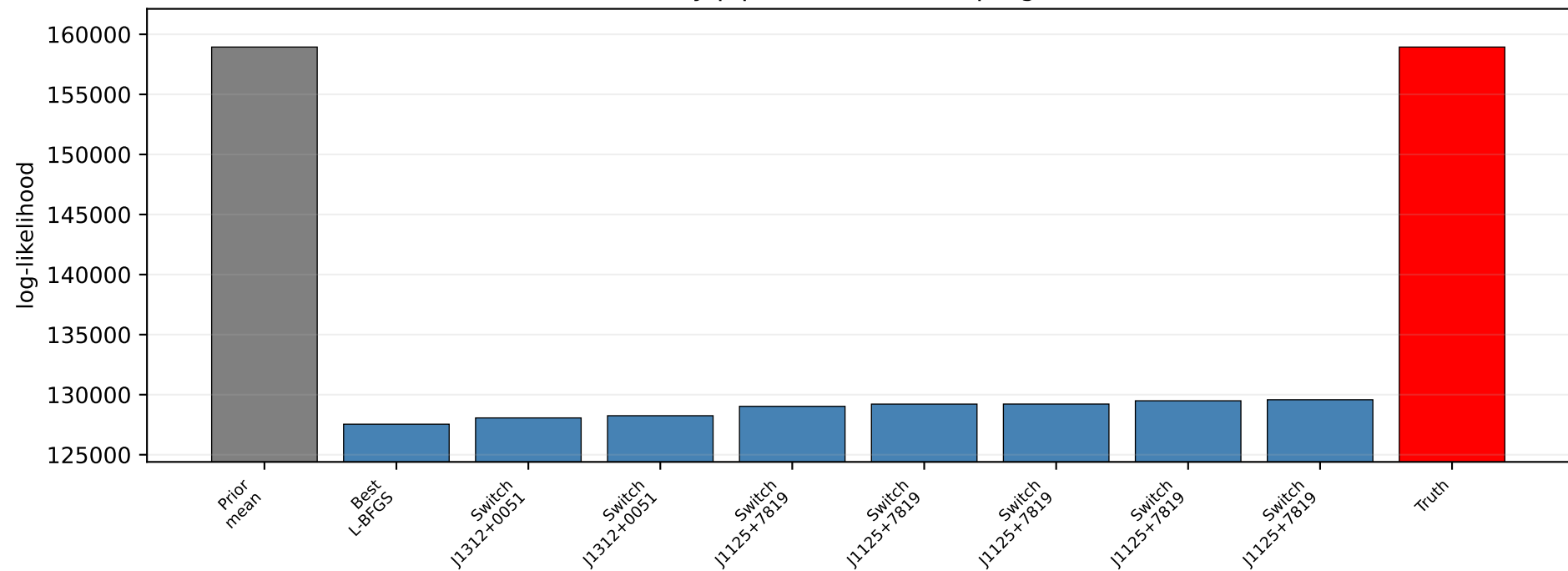
Recovery pipeline: likelihood progression
