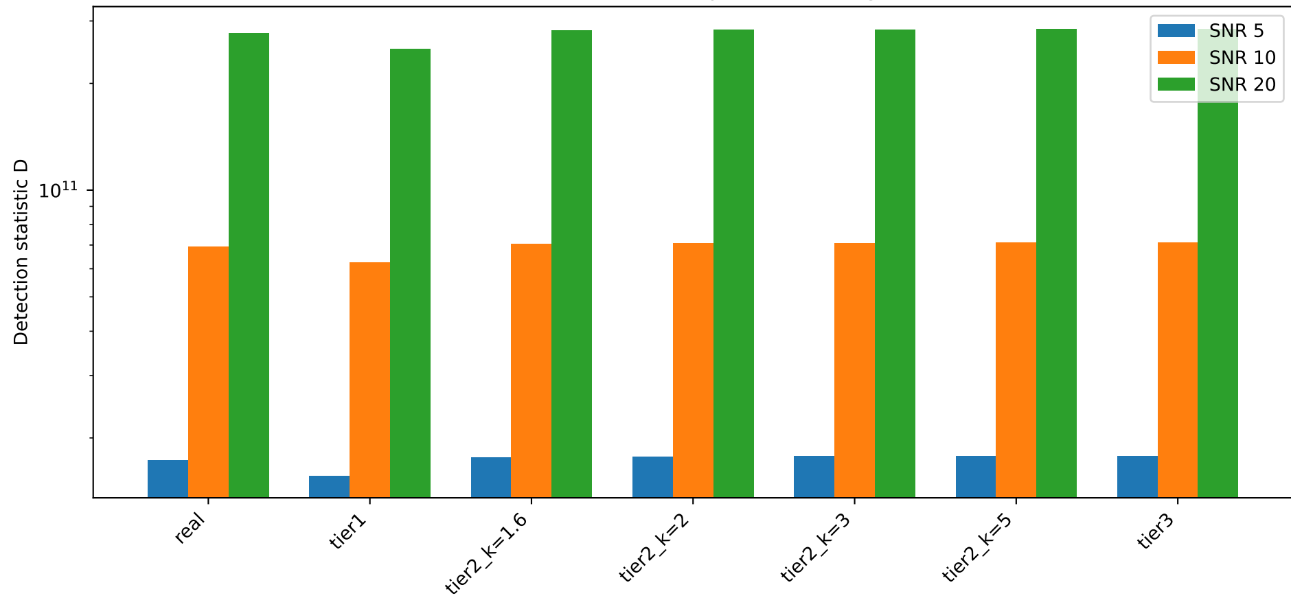
Detection statistic vs distance prior tier (marginalised CW)
