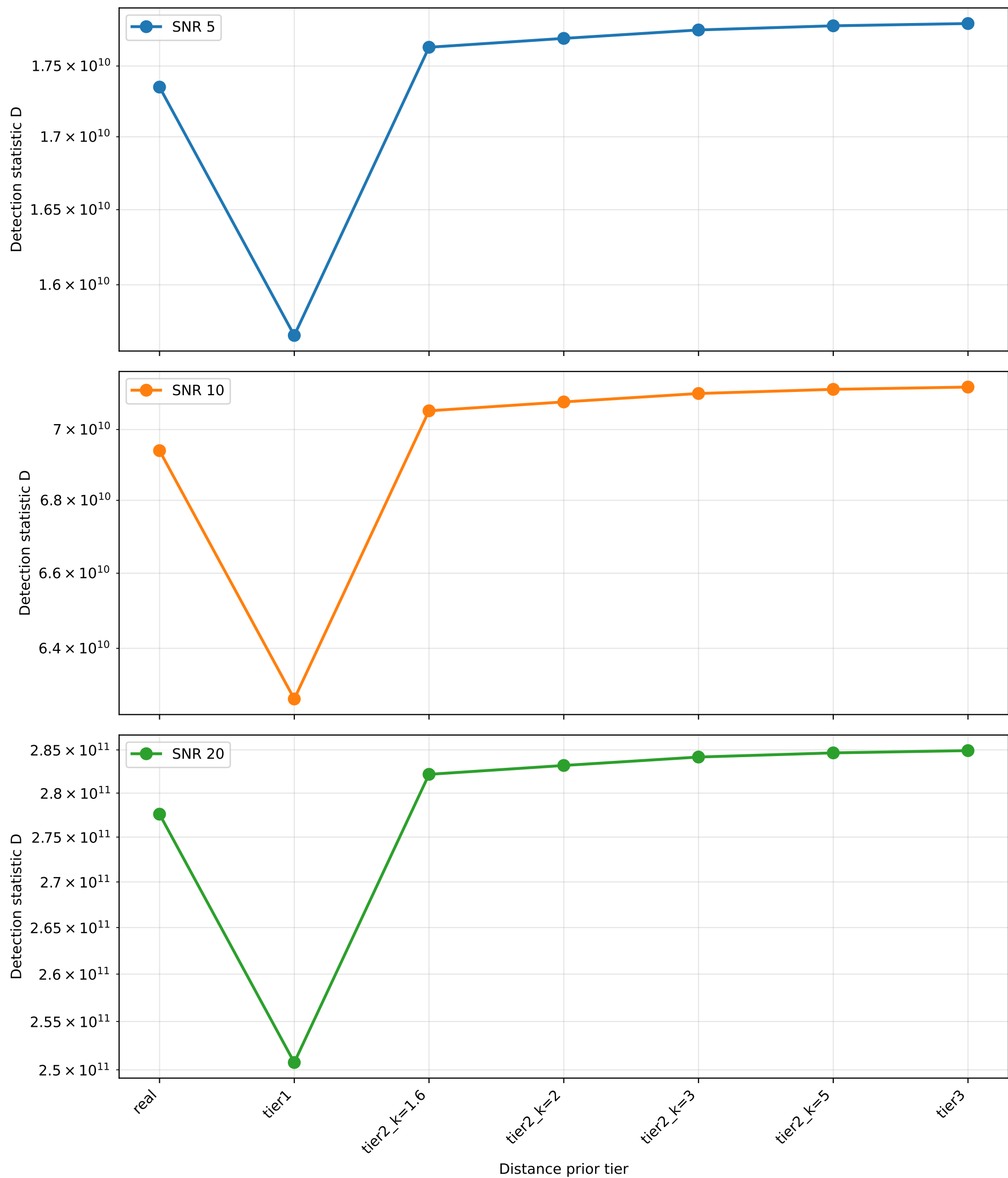
Detection Statistic Trends Across Distance Prior Tiers (log scale)
