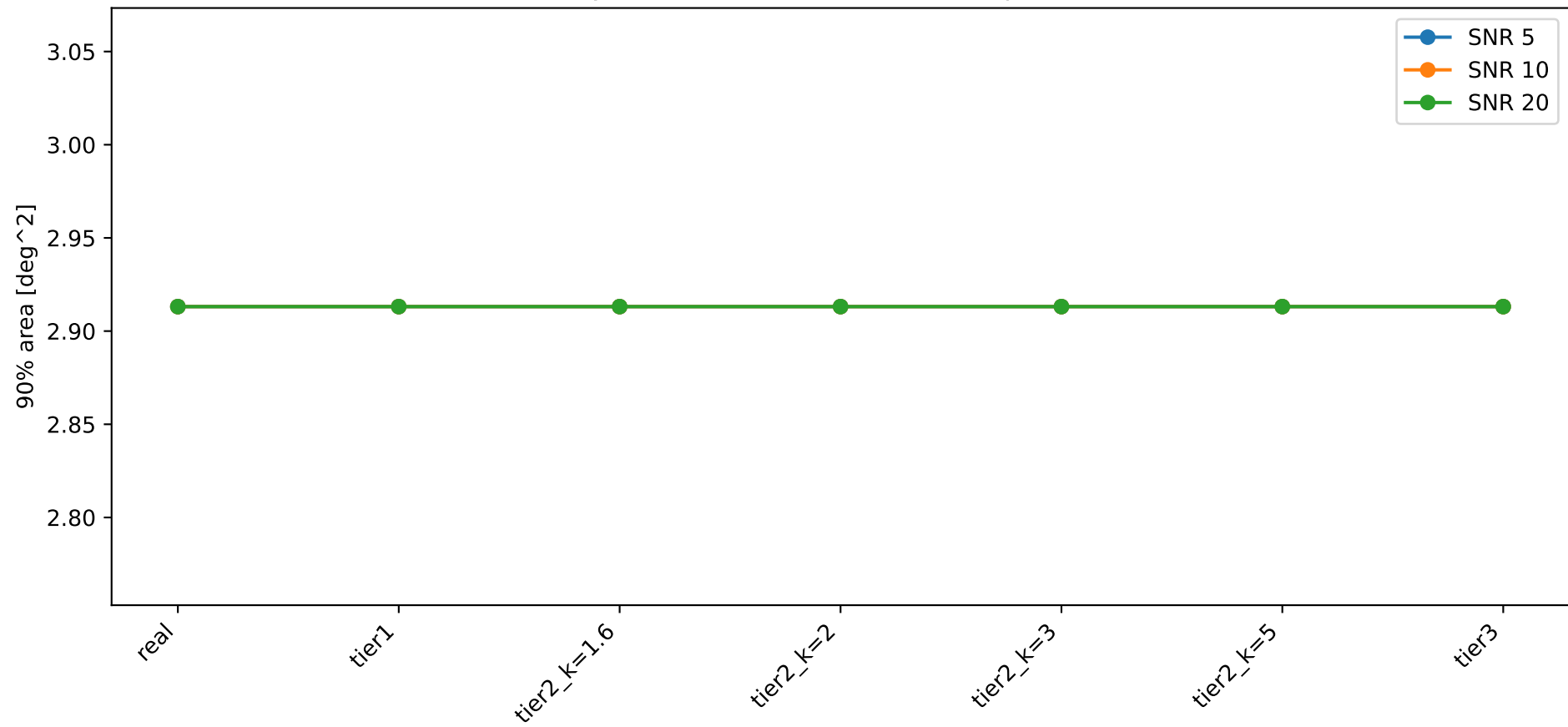
Sky localisation area vs distance prior tier
