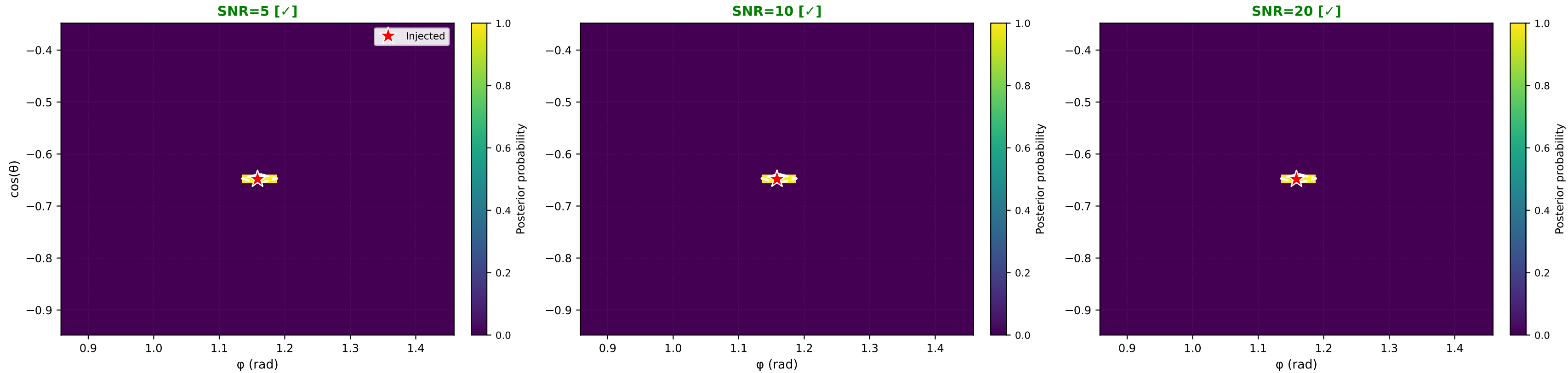
Sky Localization: real Contours: 30% (cyan), 60% (yellow), 90% (white dashed) | Red star = injected position | [ \checkmark / \times ] = inside/outside 90% CR
