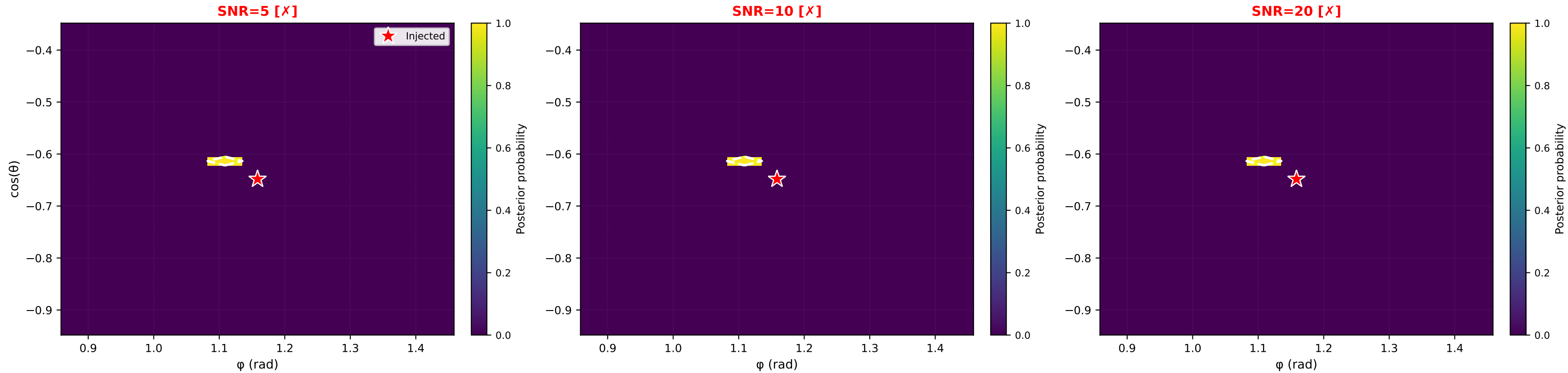
Sky Localization: tier1 Contours: 30% (cyan), 60% (yellow), 90% (white dashed) | Red star = injected position | [ \checkmark / \times ] = inside/outside 90% CR
