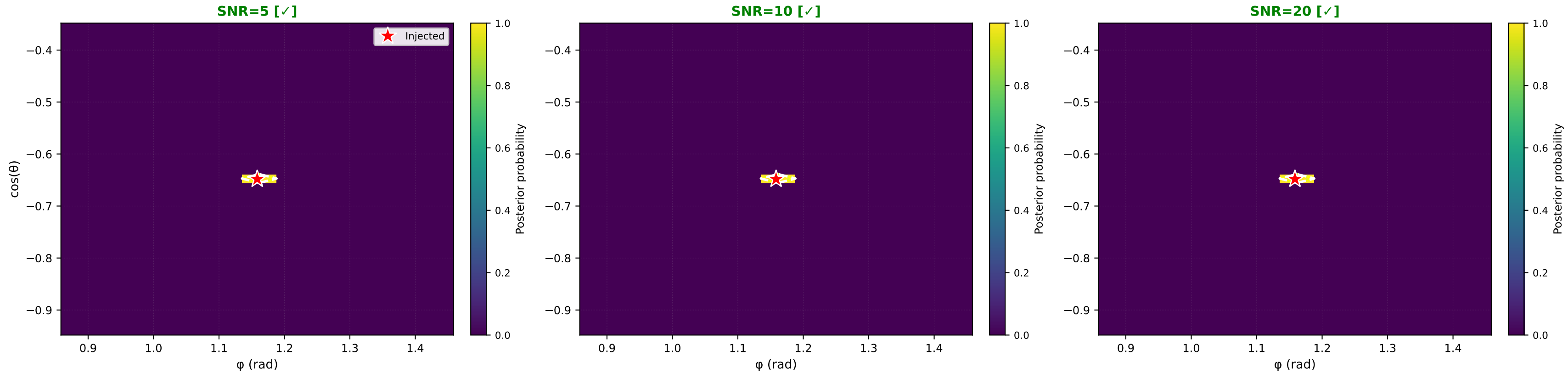
Sky Localization: tier3 Contours: 30% (cyan), 60% (yellow), 90% (white dashed) | Red star = injected position | [ \checkmark / \times ] = inside/outside 90% CR
