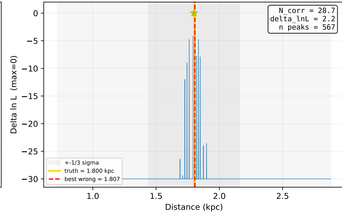
Point F: \log_{10}(M_c)=9.70 , \log_{10}(fgw)=-7.52 M_c=5e9 , f=3e-8 (realistic)
