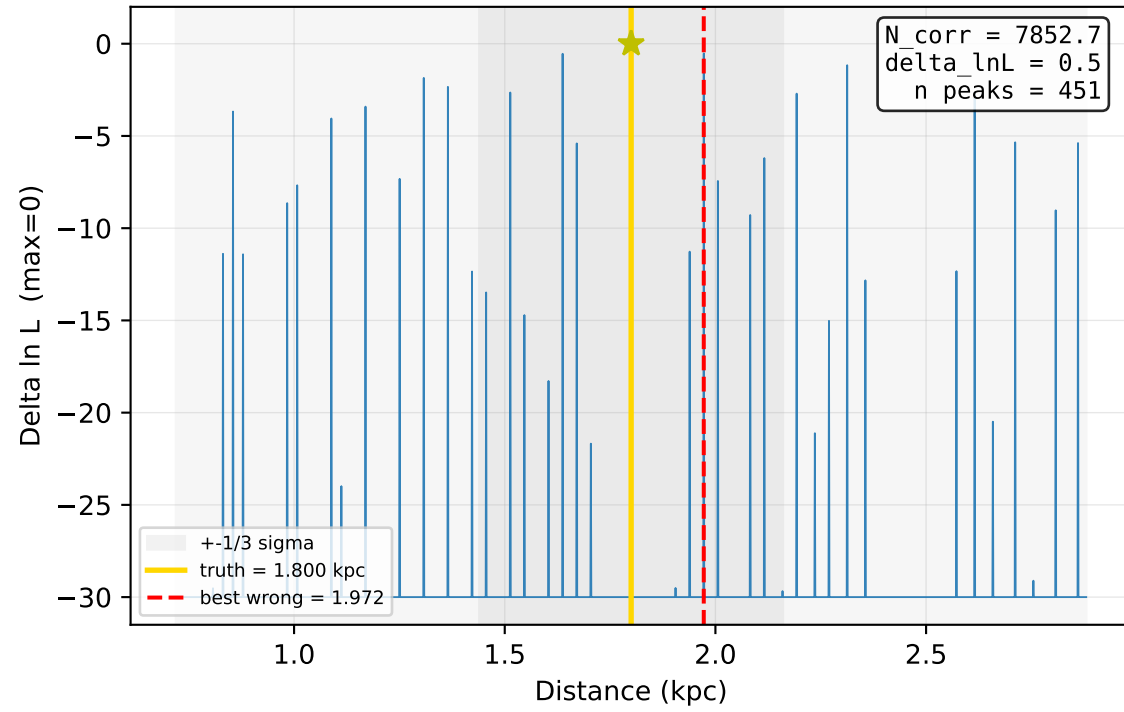
Point D: \log_{10}(M_c)=10.00 , \log_{10}(fgw)=-7.00 N < 1 , strong evol
