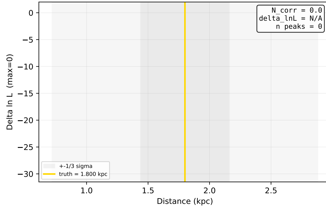
Point E: \log_{10}(M_c)=11.00 , \log_{10}(fgw)=-7.00 N \ll 1 , extreme evol
