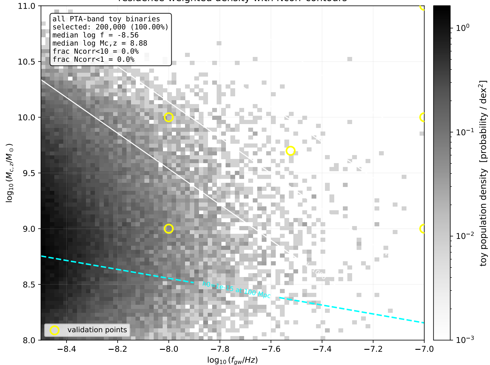
Part F1: All toy SMBHBs in the PTA band residence-weighted density with Ncorr contours
