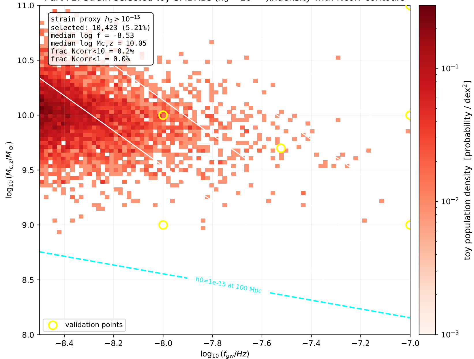
Part F2: Strain-selected toy SMBHBs ( h_0 > 10^{-15} ) density with Ncorr contours
