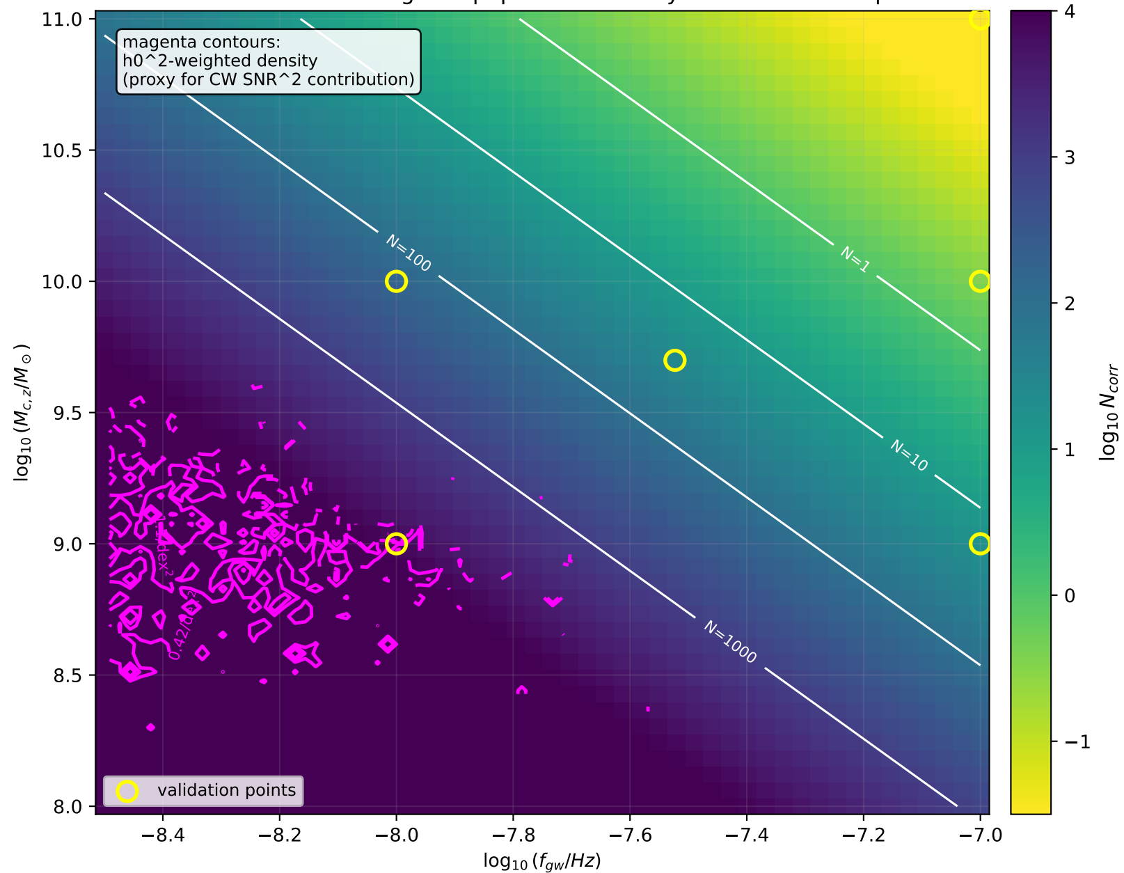
Part F3: Strain-weighted population density on Ncorr heatmap
