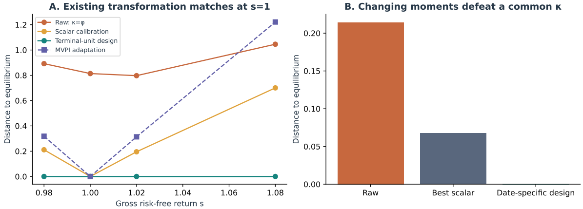
Figure 2: NUMERICALLY VERIFIED. Existing MVPI adaptation agrees at zero interest but targets per-step mean-volatility away from it. With changing moments at zero interest, a common scalar penalty leaves distance 0.067715; the date-specific design gives zero.
