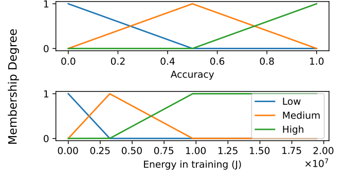
Fig. 13. Membership functions for energy consumptions during training and accuracy for MLP on MNIST from BUTTER-E.
