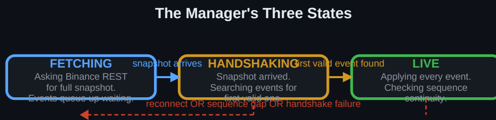
Figure 16 - Any failure from any state resets to Fetching. There is no partial recovery.
