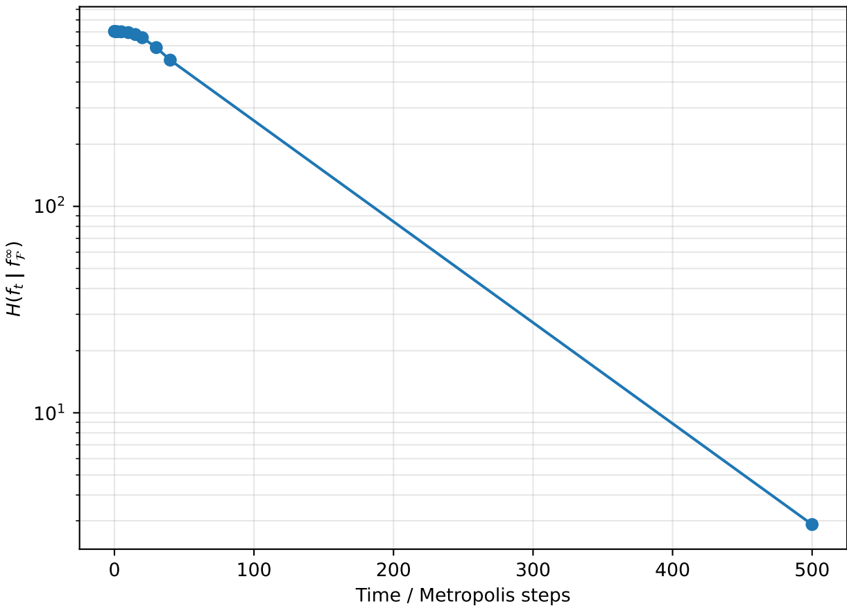
Relative-entropy decay at fixed T = 5.0
